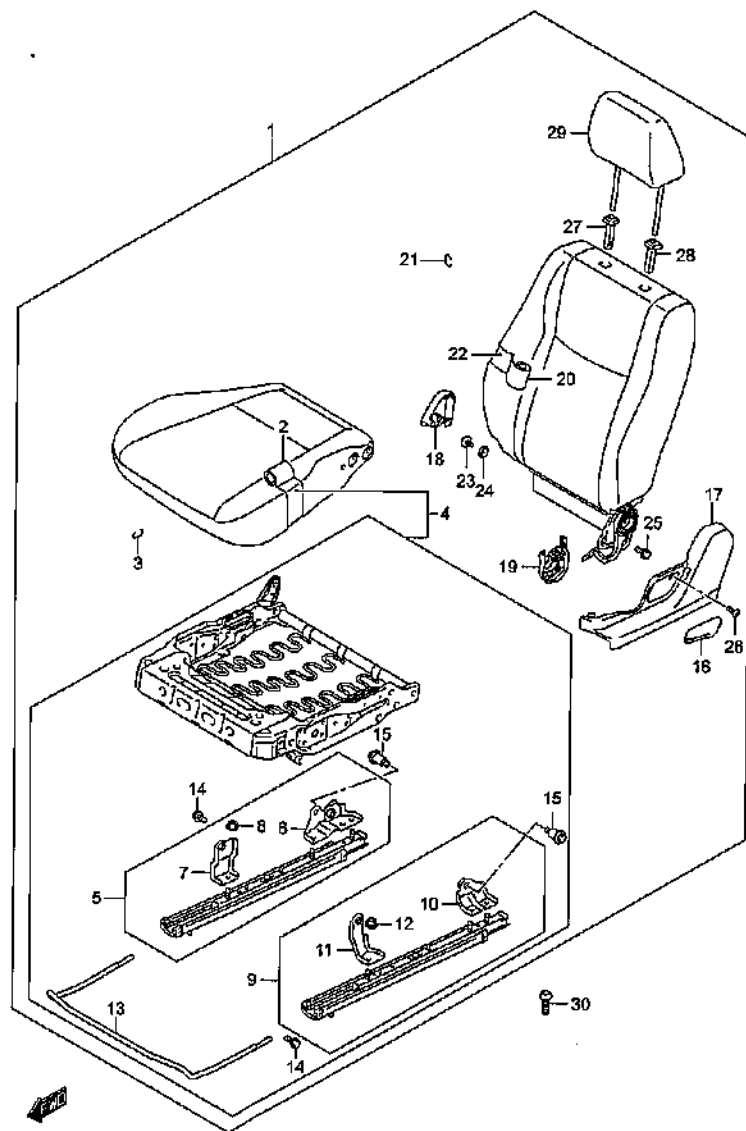
FRONT LH SEAT
