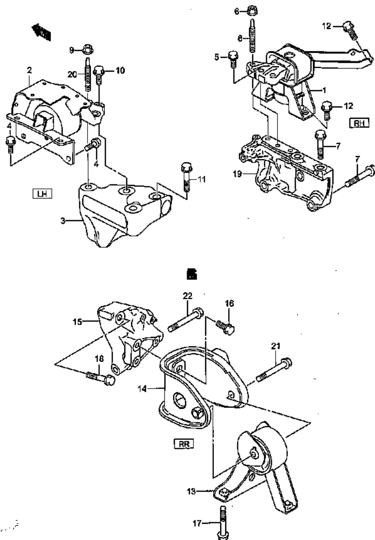
ENGINE MOUNTING (2)
