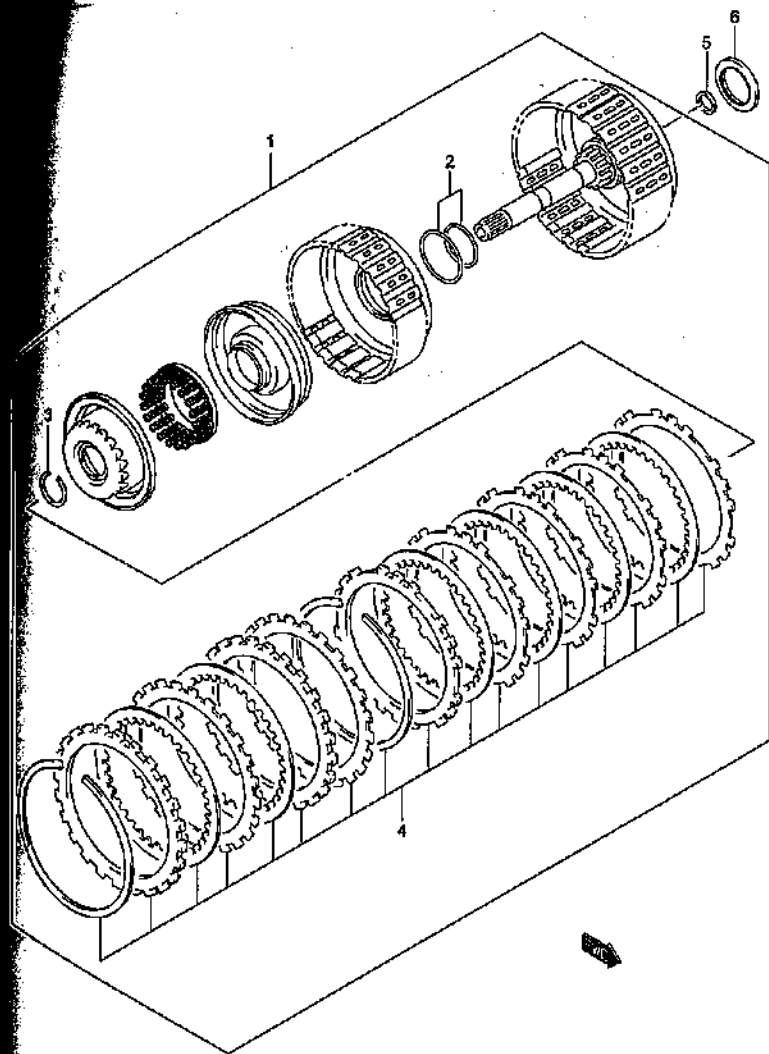
AT FORWARD CLUTCH
