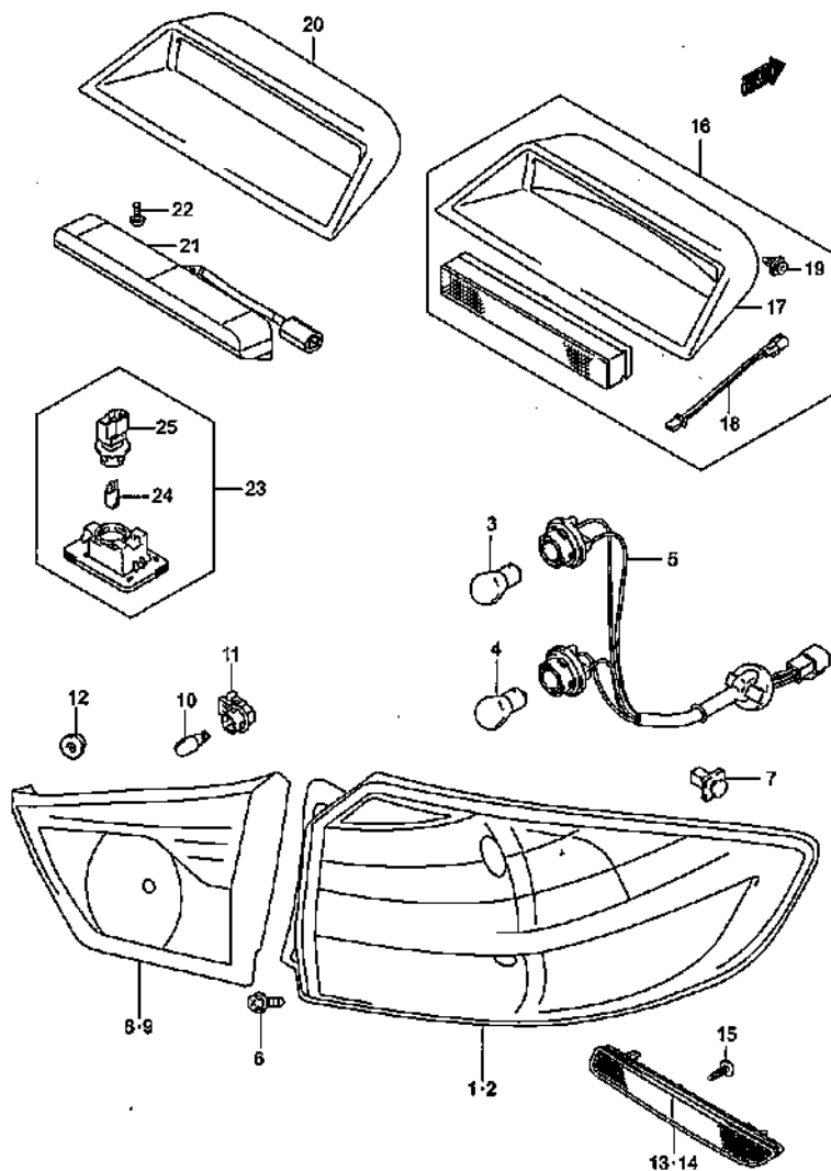
REAR LAMP (1)
