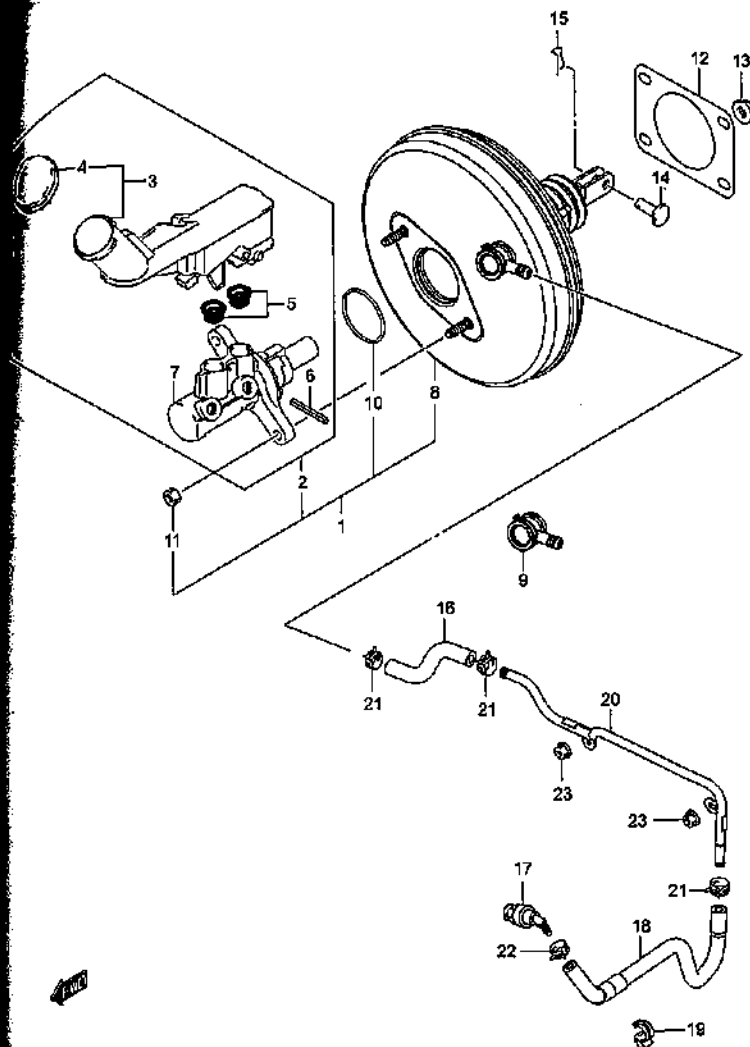
BRAKE MASTER CYLINDER (5)
