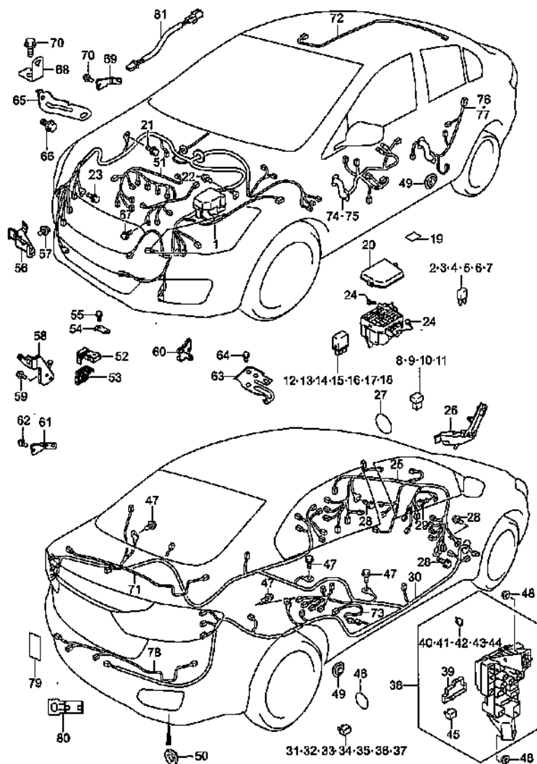
WIRING HARNESS (1)
