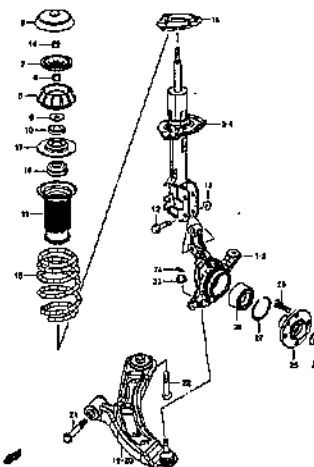
FRONT SUSPENSION
