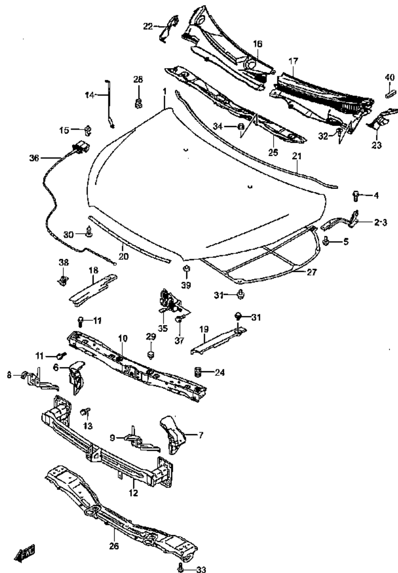
FRONT HOOD PANEL
