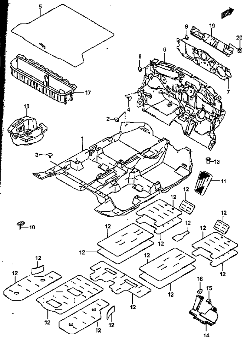
FLOOR CARPET
