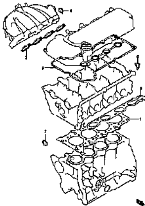
ENGINE GASKETS (1)
