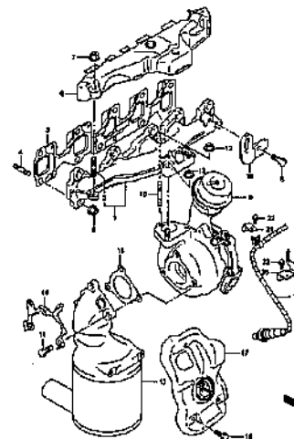
EXHAUST MANIFOLD (3)
