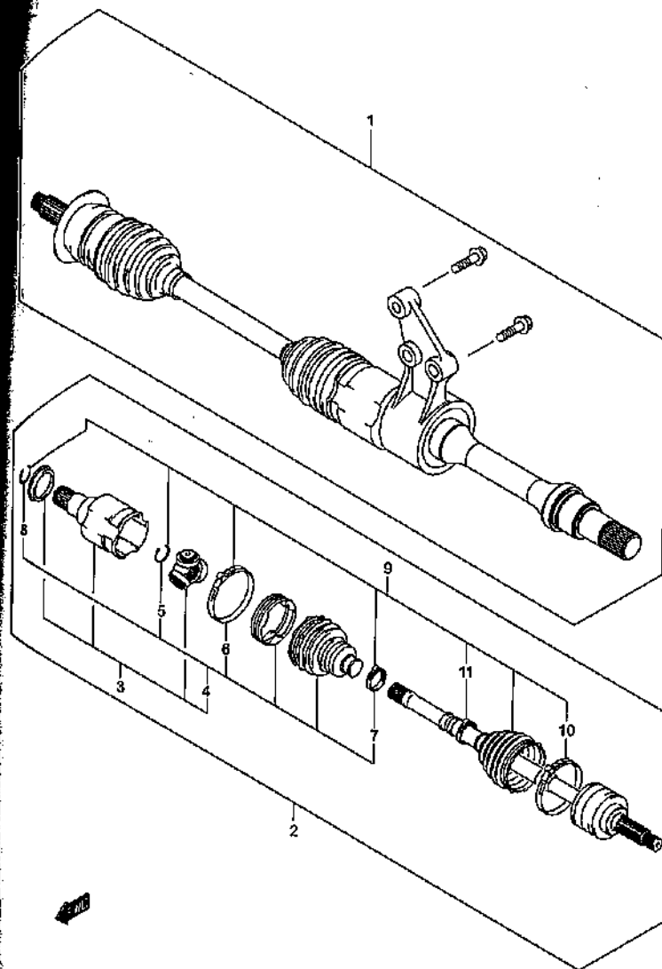
FRONT DRIVE SHAFT (4)
