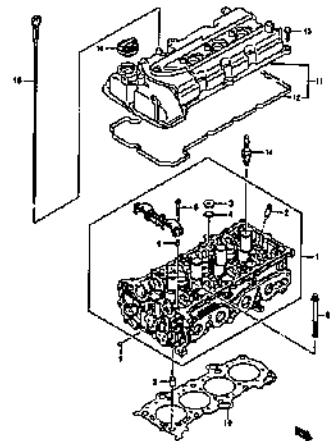
CYLINDER HEAD (1)
