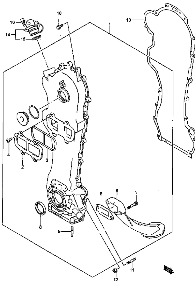
OIL PUMP (2)
