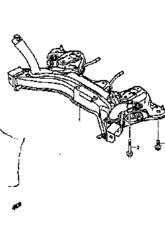
FRONT SUSPENSION FRAME
