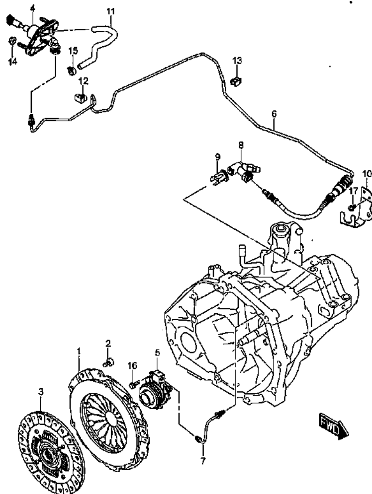
MT CLUTCH (2)
