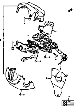
STEERING COLUMN (1)
