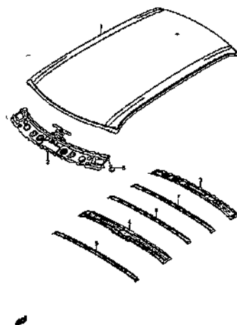
ROOF PANEL
