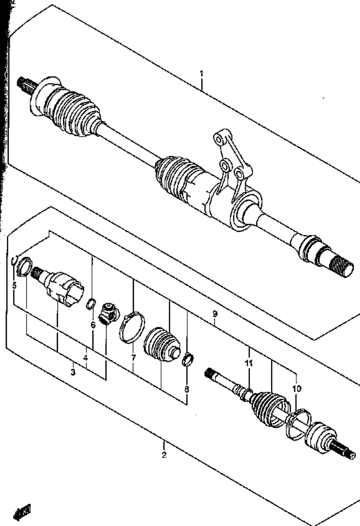
FRONT DRIVE SHAFT (1)
