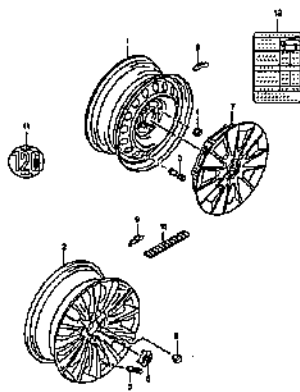
ROAD WHEEL/TIRE (2)
