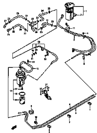
FUEL PUMP (2)
