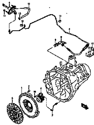
MT CLUTCH (4)
