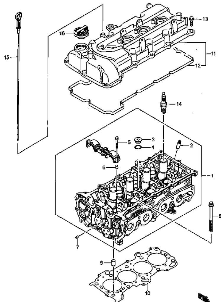
CYLINDER HEAD (2)
