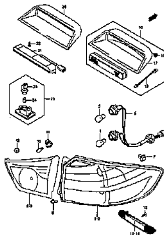
REAR LAMP (1)
