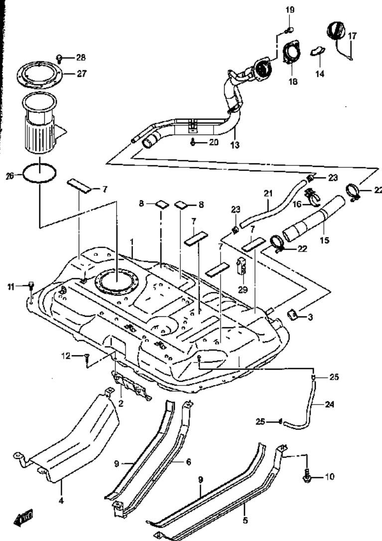
FUELTANK (1)
