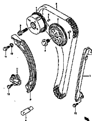
CAM CHAIN (1)
