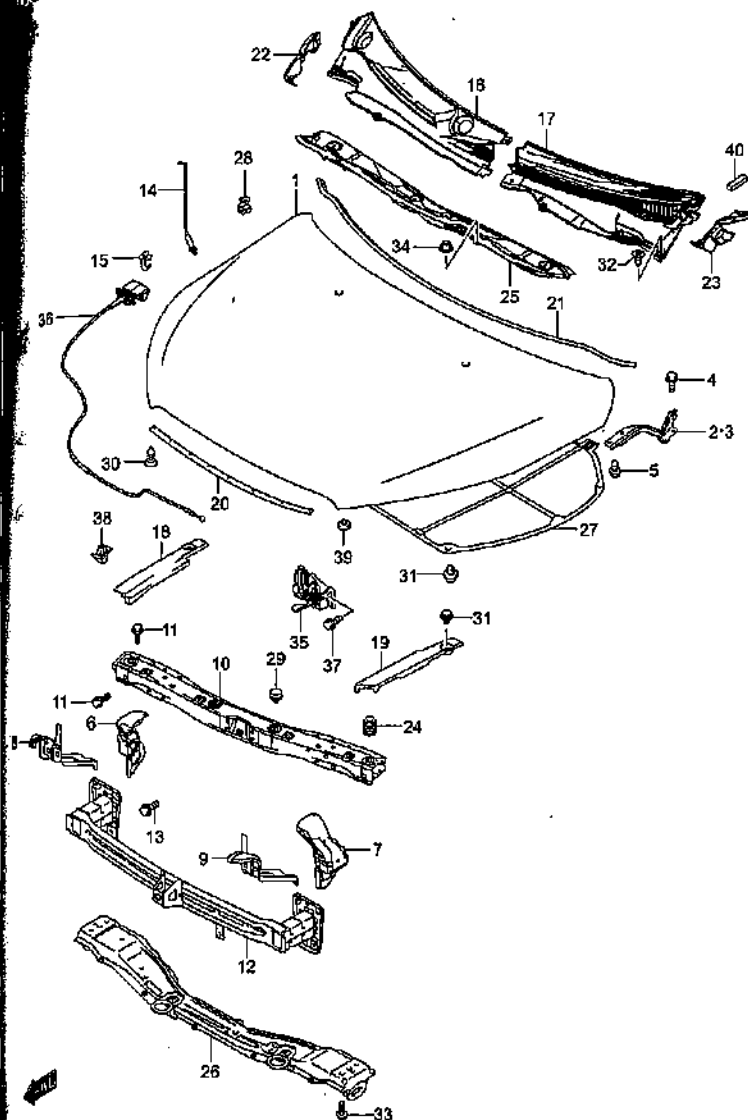
FRONT HOOD PANEL
