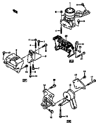
ENGINE MOUNTING (2)
