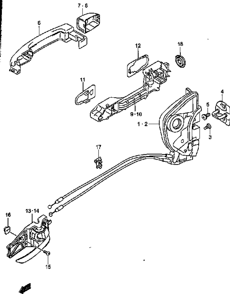
FRONT DOOR LOCK
