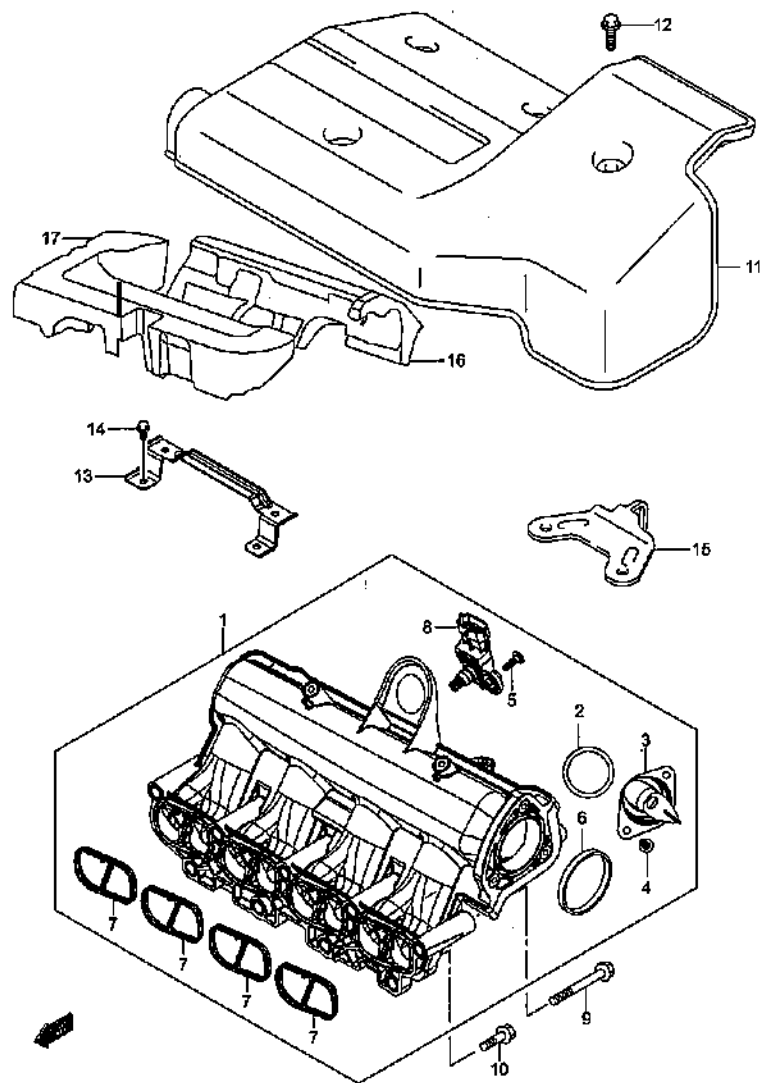
INTAKE MANIFOLD (2)
