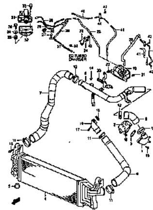
INTER COOLER
