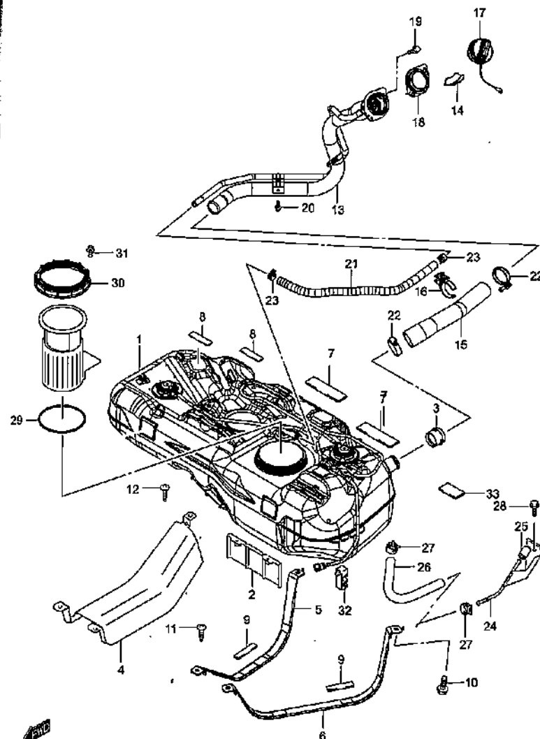
FUELTANK (2)
