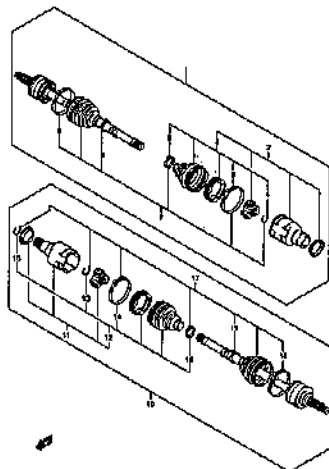
FRONT DRIVE SHAFT (6)
