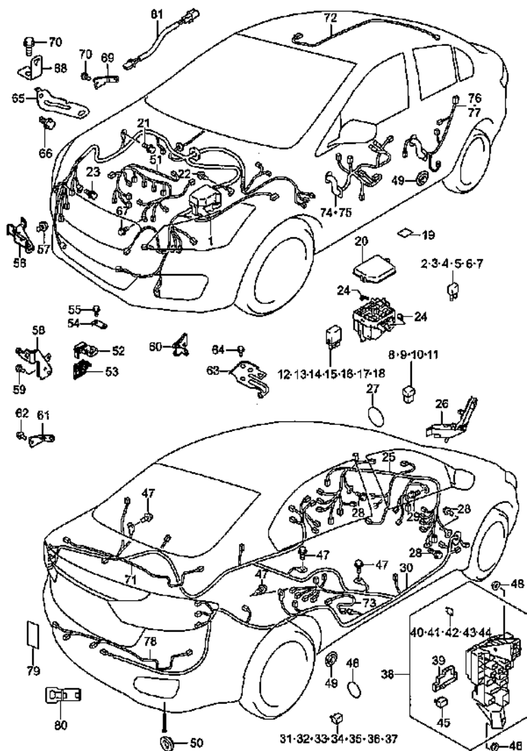
WIRING HARNESS (1)
