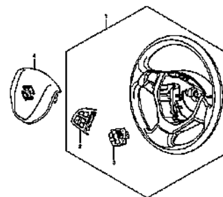
STEERING WHEEL (2)
