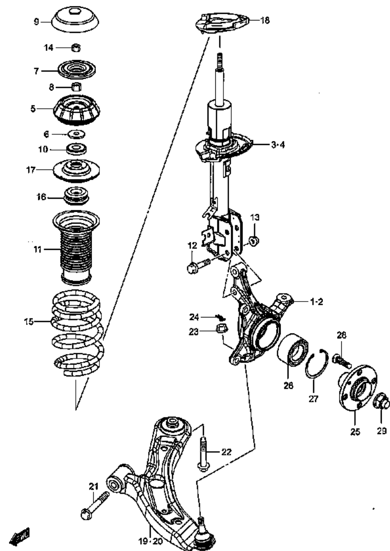
FRONT SUSPENSION
