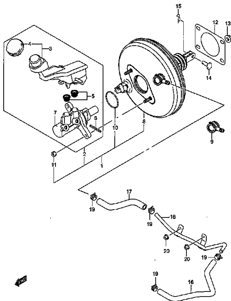
BRAKE MASTER CYLINDER (4)
