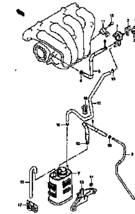
EMISSION CONTROL (1)
