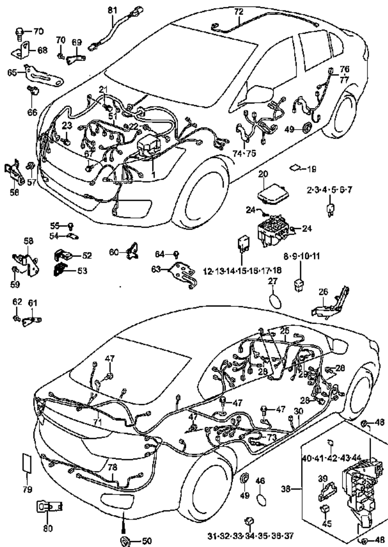
WIRING HARNESS (1)
