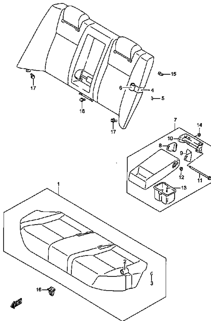
REAR SEAT
