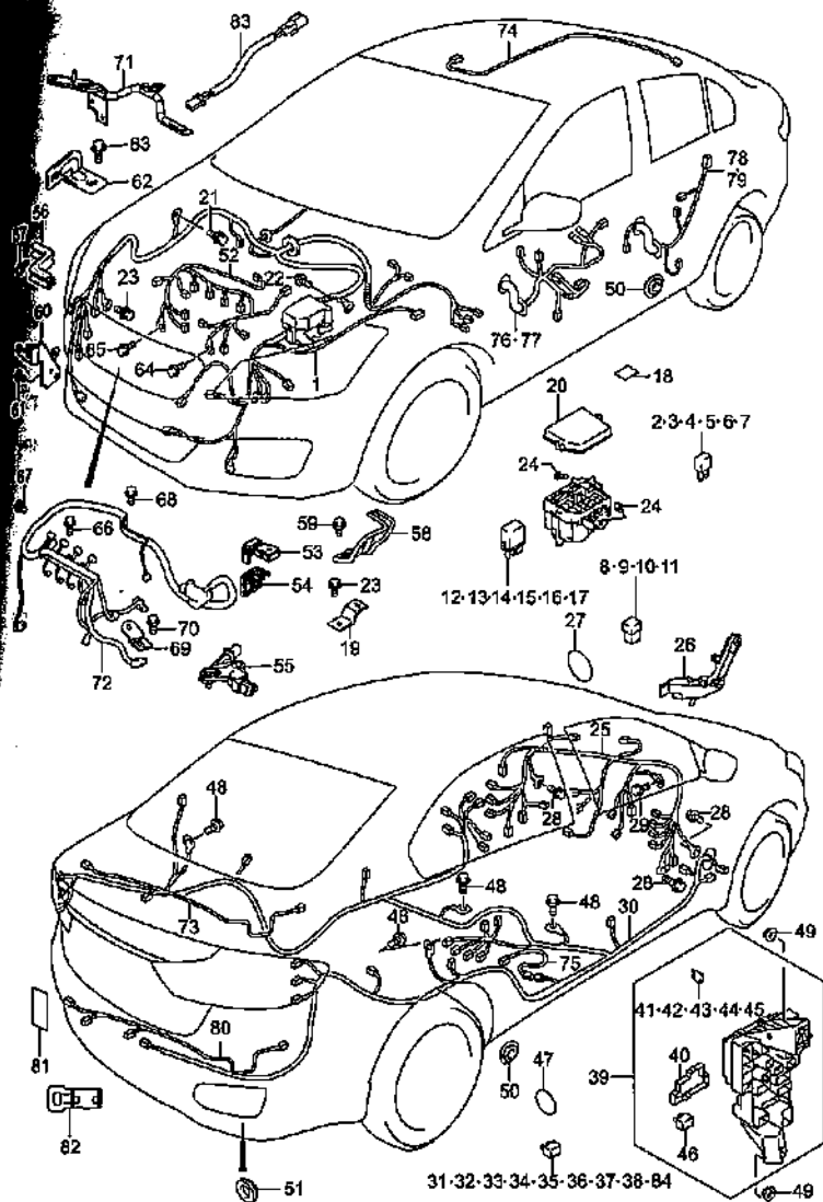
WIRING HARNESS (3)
