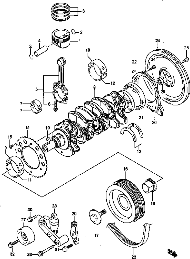
CRANKSHAFT (2)
