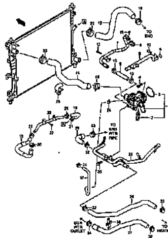
WATER HOSE (3)
