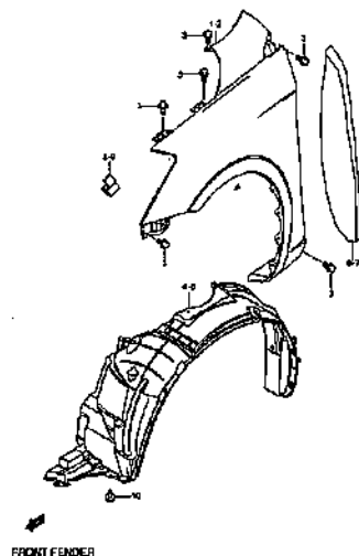
FRONT FENDER
