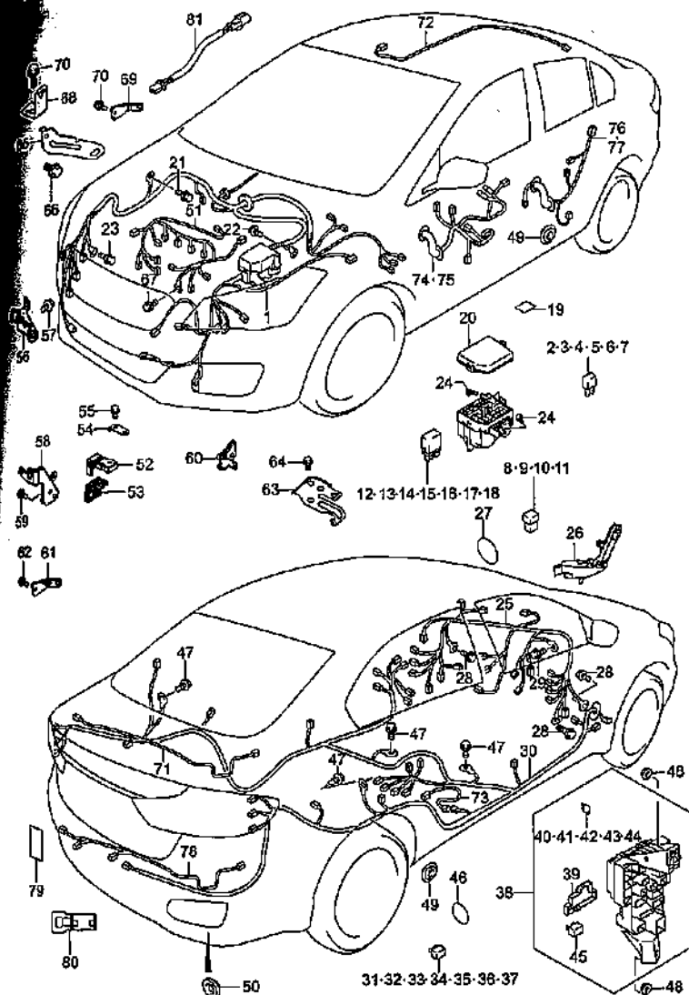
WIRING HARNESS (1)
