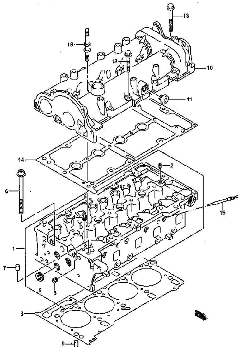
CYLINDER HEAD
