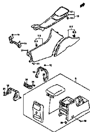
CONSOLE BOX
