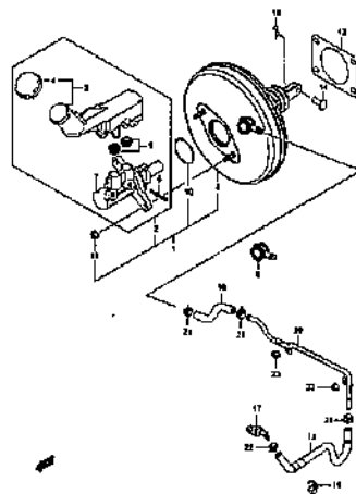
BRAKE MASTER CYLINDER (5)
