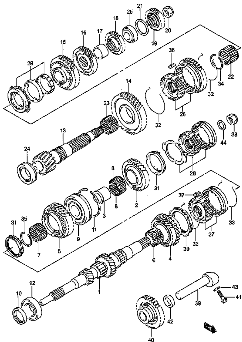
MT TRANSMISSION GEAR (1)
