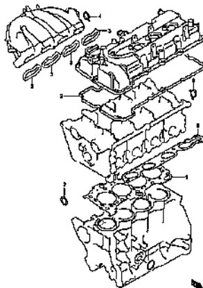
ENGINE GASKETS (2)
