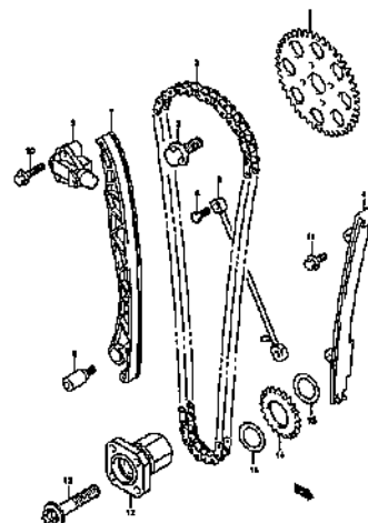
CAM CHAIN (3)
