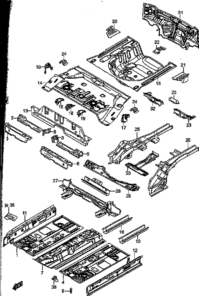
FLOOR PANEL
