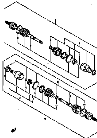
FRONT DRIVE SHAFT (2)
