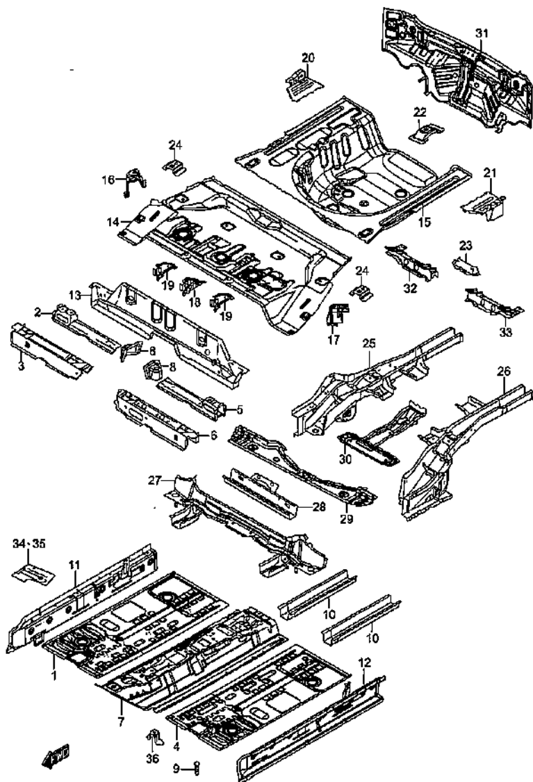
FLOOR PANEL
