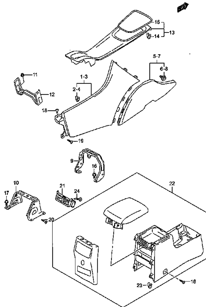
CONSOLE BOX
