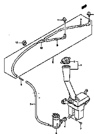
WINDOW WASHER
