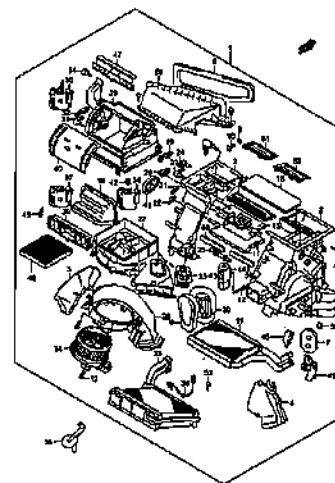
HEATER
