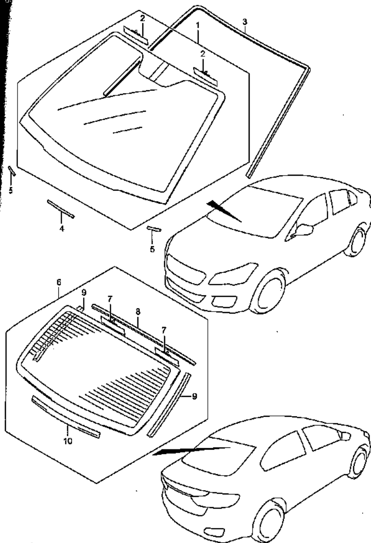
FRONT/BACK GLASS
