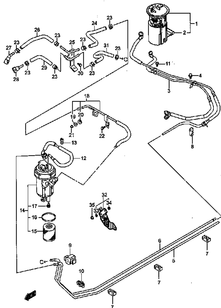
FUEL PUMP (2)
