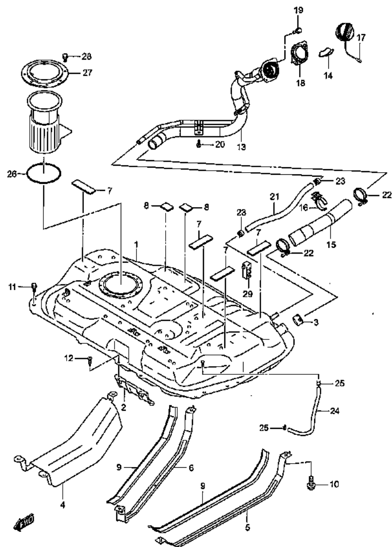
FUELTANK (1)
