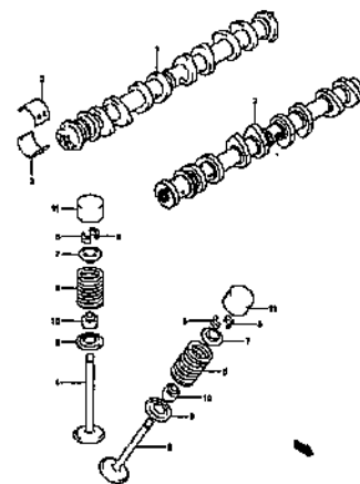
CAM SHAFT/VALVE (1)
