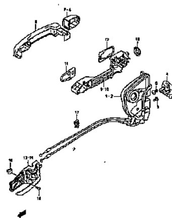
FRONT DOOR LOCK
