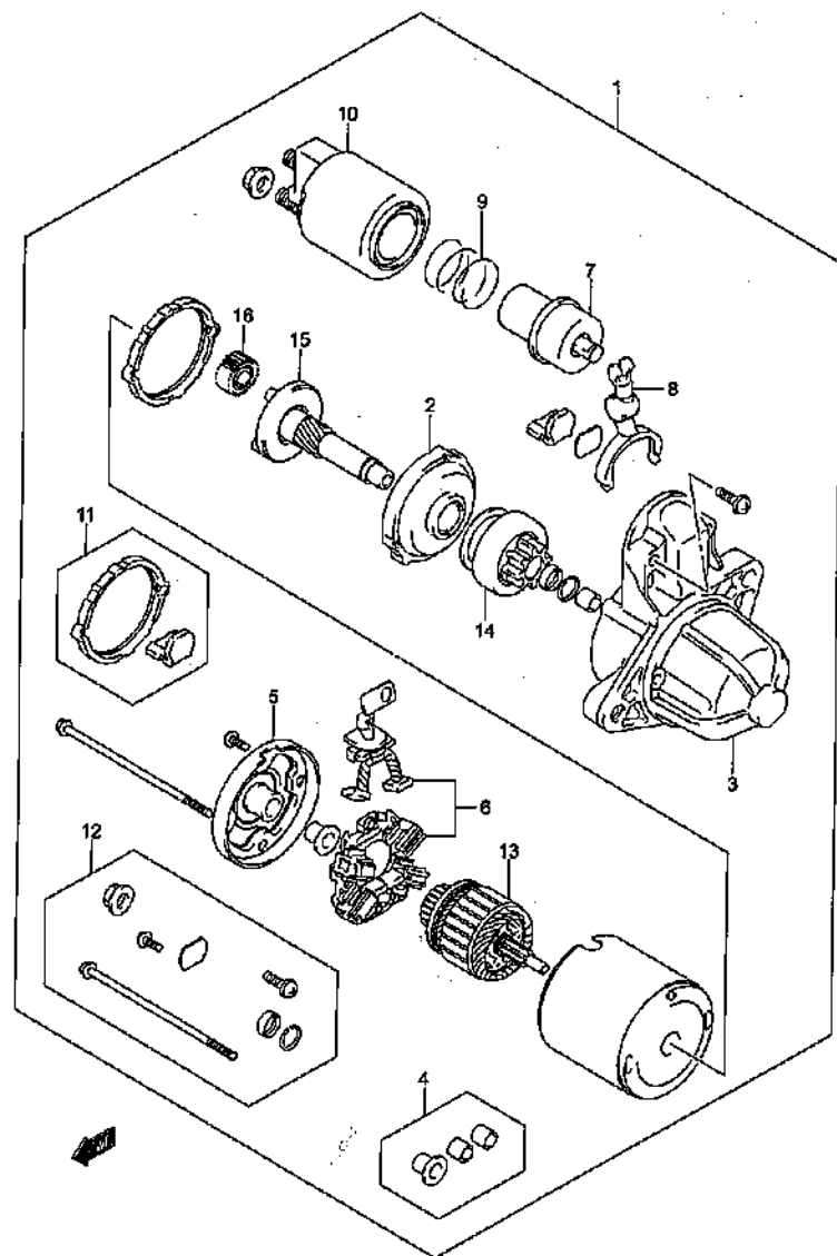
STARTING MOTOR (2)
