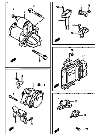
ENGINE ELECTRICAL (2)
