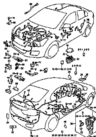
WIRING HARNESS (2)
