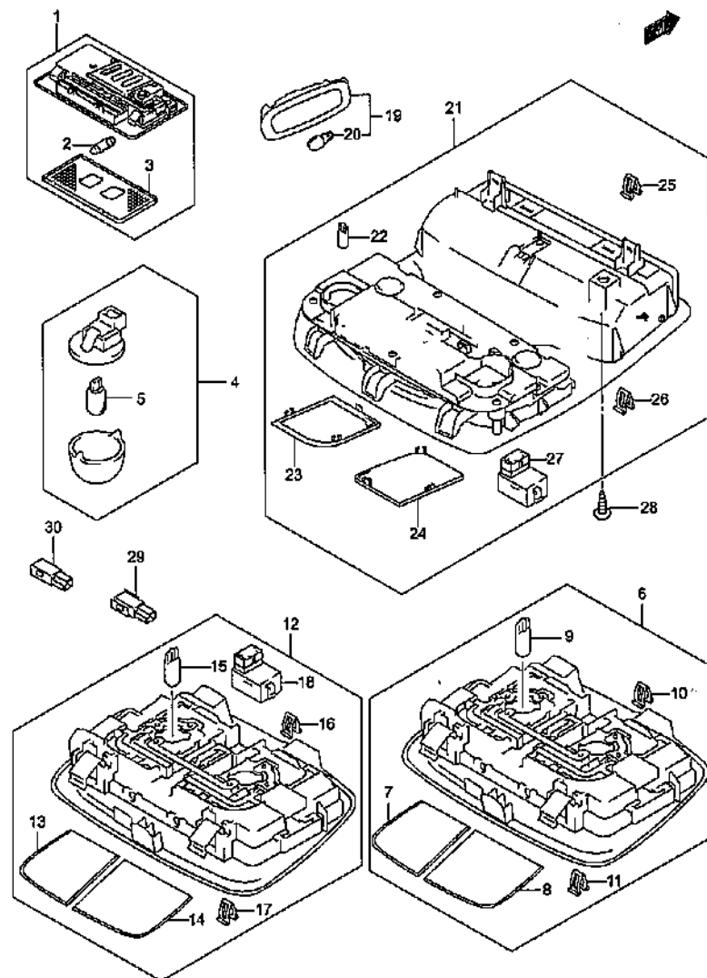
ROOM LAMP
