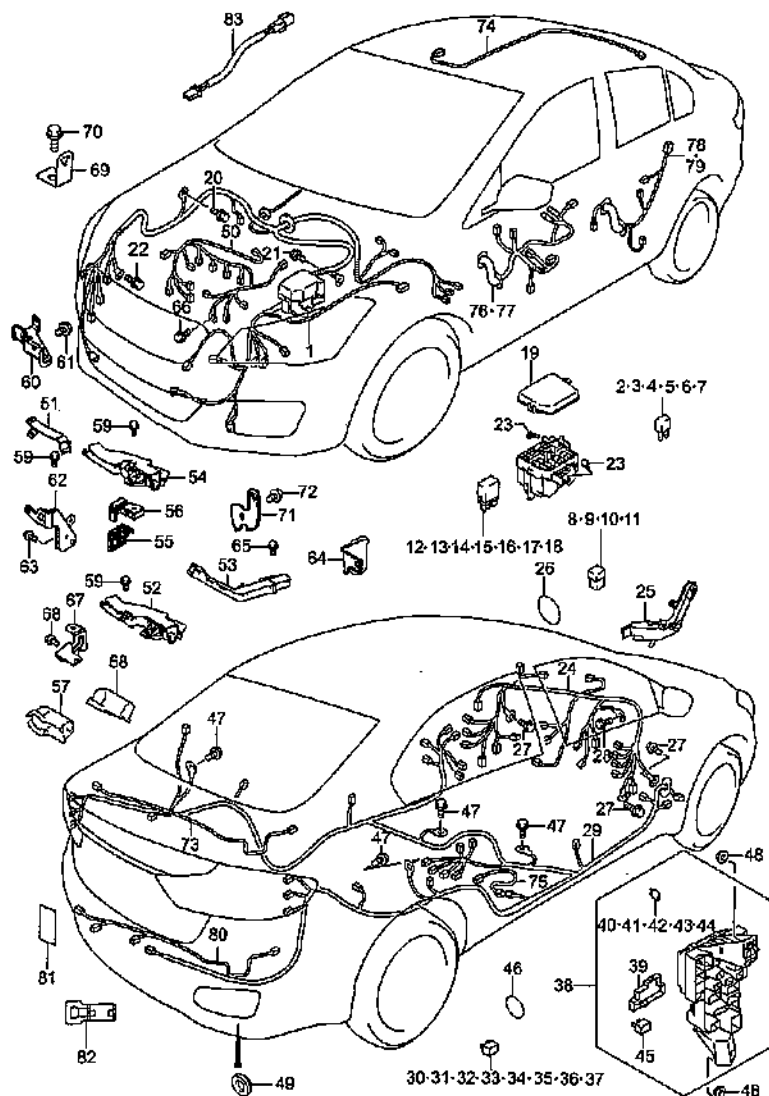
WIRING HARNESS (2)
