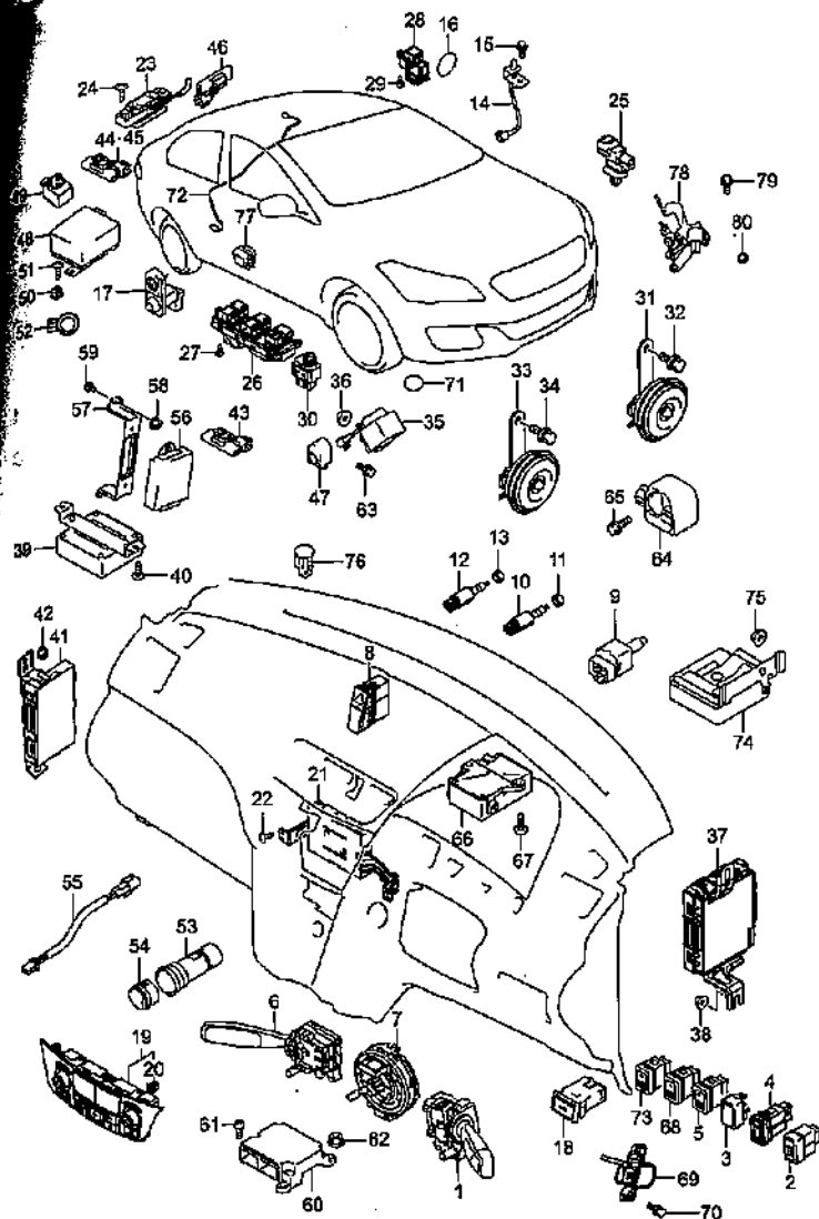
ELECTRICAL CONTROL
