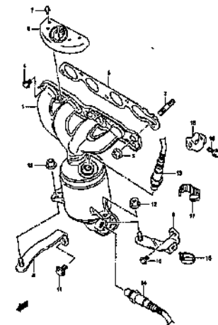
EXHAUST MANIFOLD (2)
