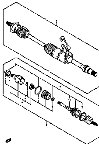
FRONT DRIVE SHAFT (1)
