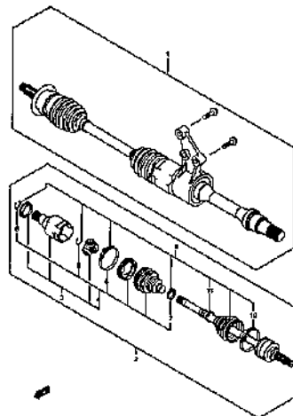
FRONT DRIVE SHAFT (5)
