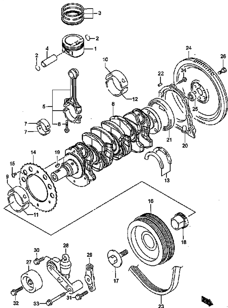
CRANKSHAFT (2)
