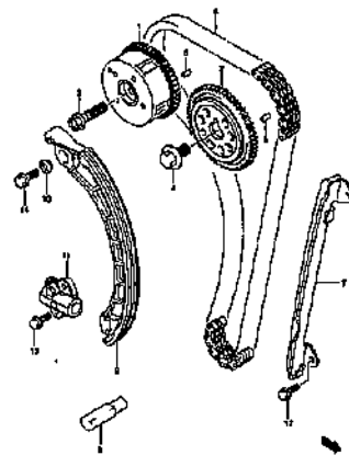
CAM CHAIN (2)
