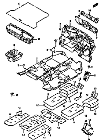
FLOOR CARPET
