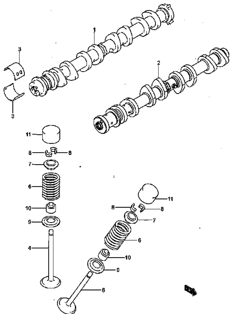
CAM SHAFT/VALVE (1)
