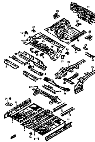
FLOOR PANEL
