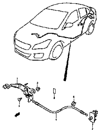
FUEL LID OPENER
