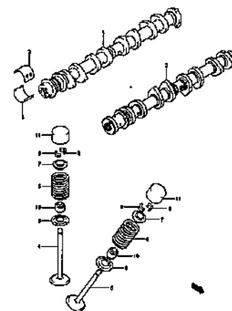
CAM SHAFT/VALVE (2)
