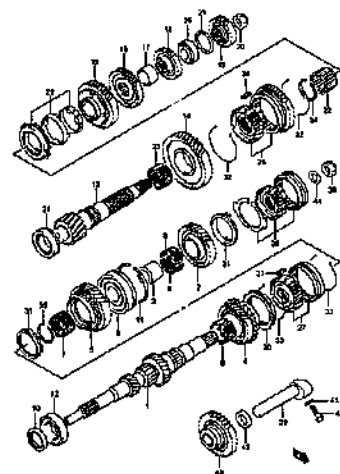
MT TRANSMISSION GEAR (1)
