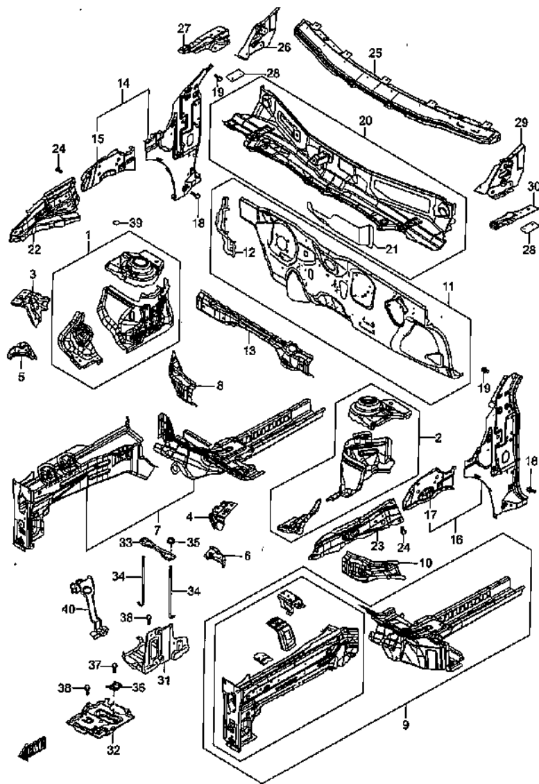
FRONT BODY PANEL
