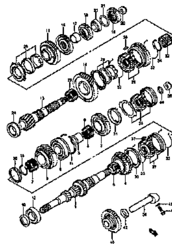
MT TRANSMISSION GEAR (2)
