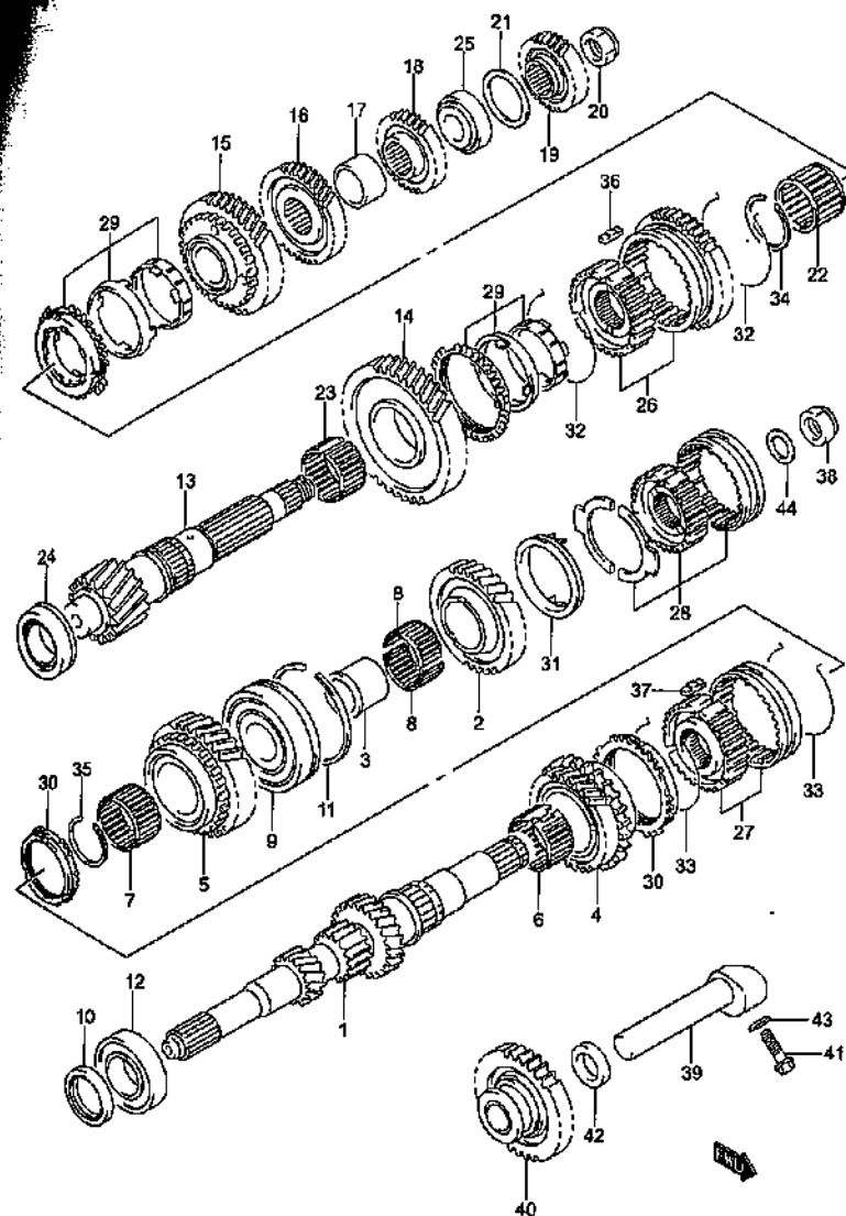
MT TRANSMISSION GEAR (2)
