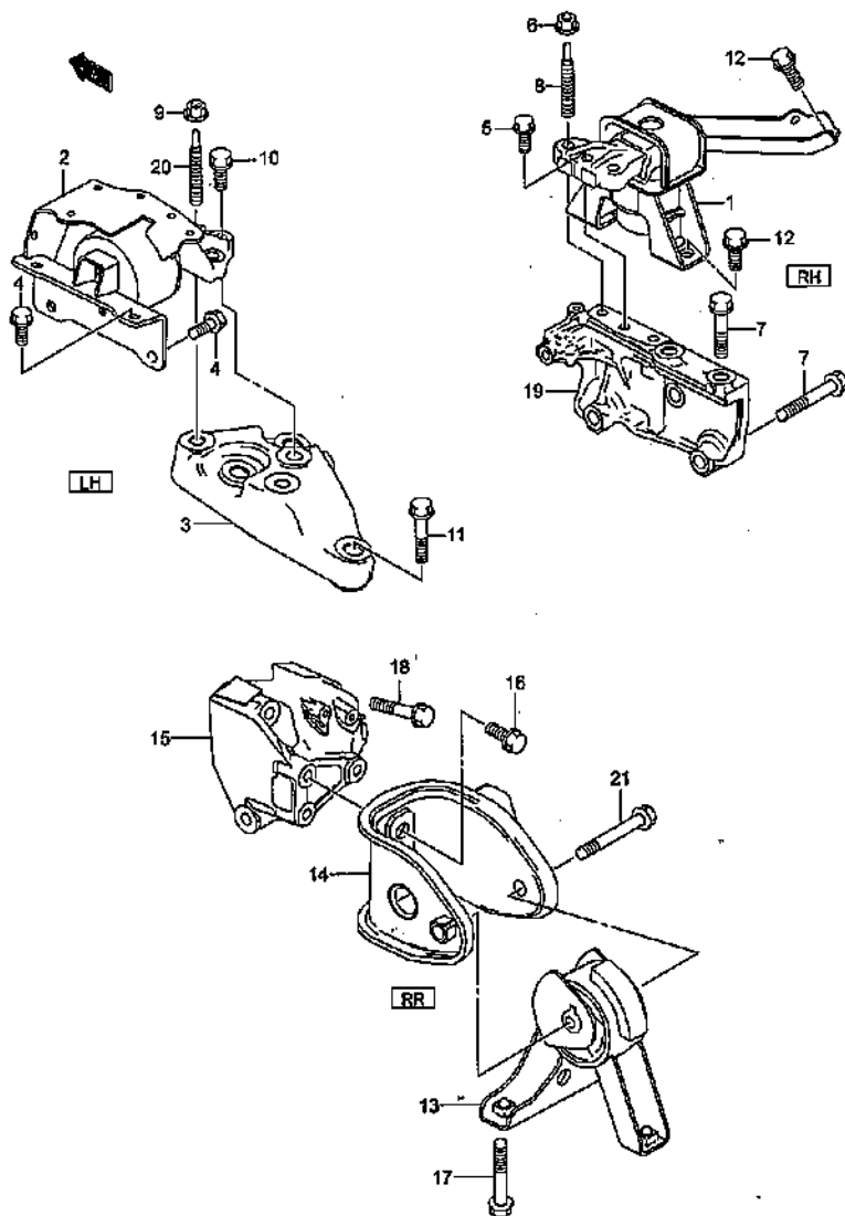
ENGINE MOUNTING (2)
