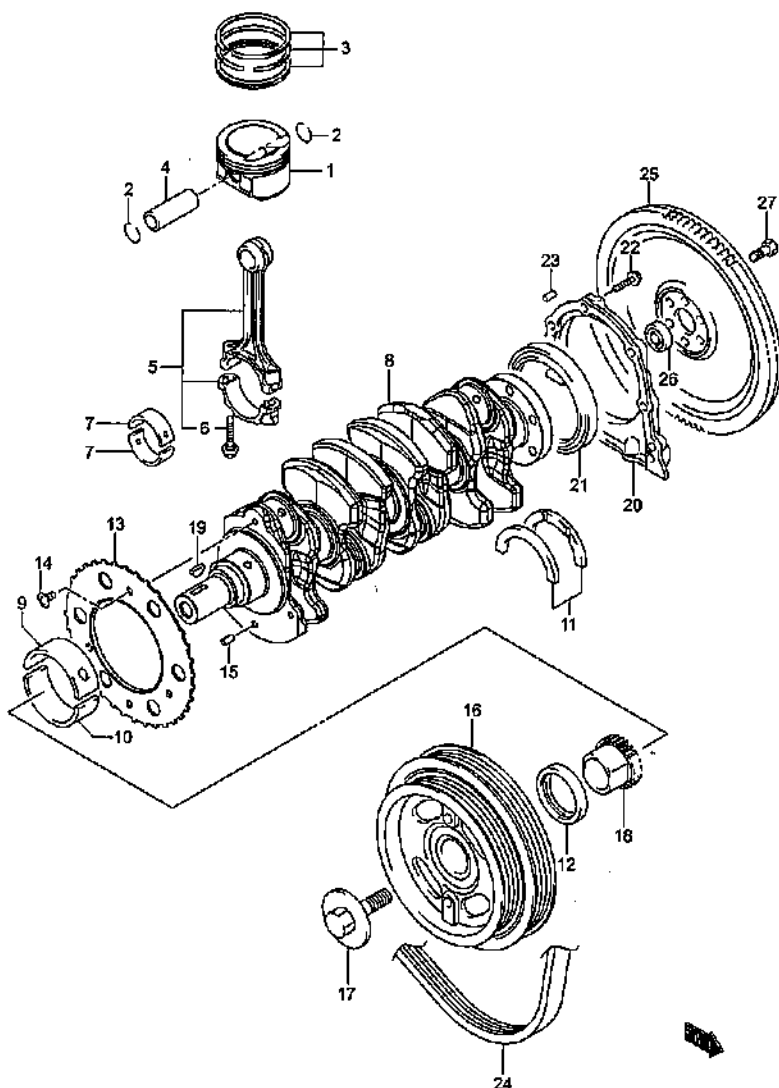
CRANKSHAFT (1)
