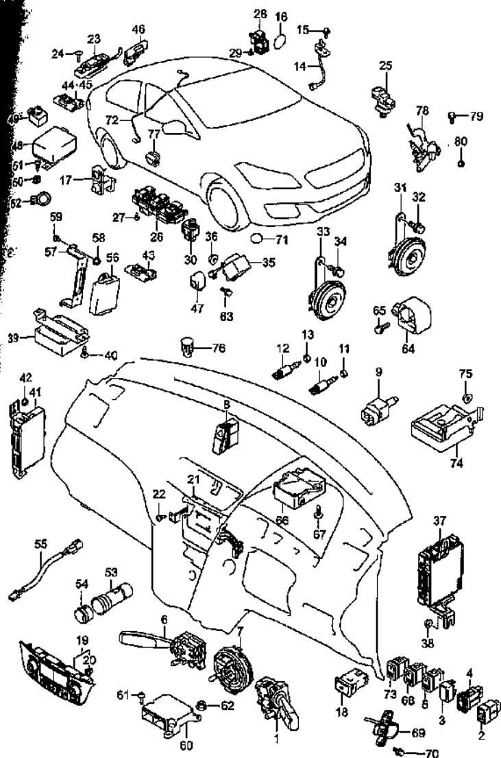
ELECTRICAL CONTROL
