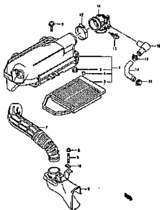
AIR CLEANER (2)
