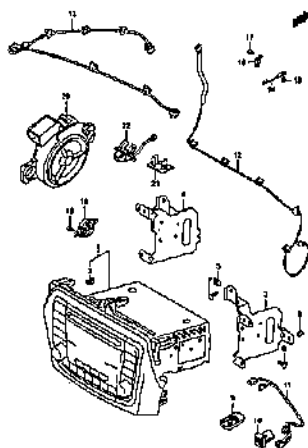
RADIO (2)
