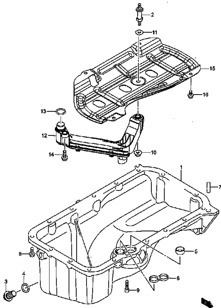
OILPAN (2)
