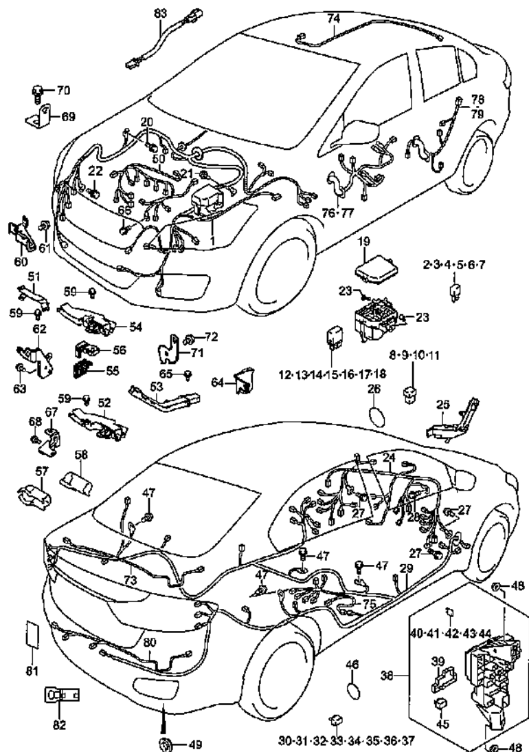
WIRING HARNESS (2)
