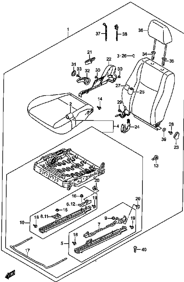
FRONT RH SEAT
