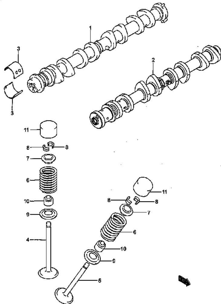
CAM SHAFT/VALVE (1)
