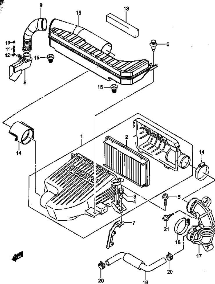
AIR CLEANER (1)
