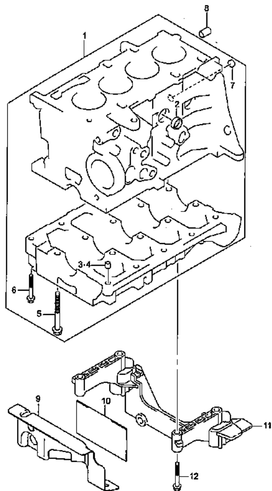
CYLINDER
