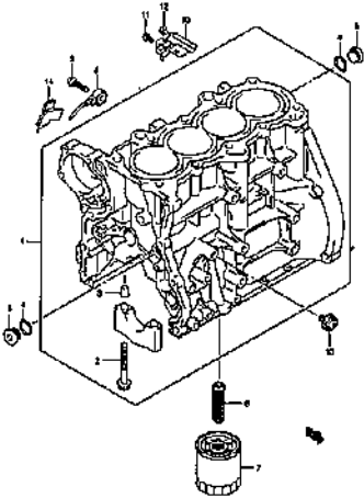
CYLINDER
