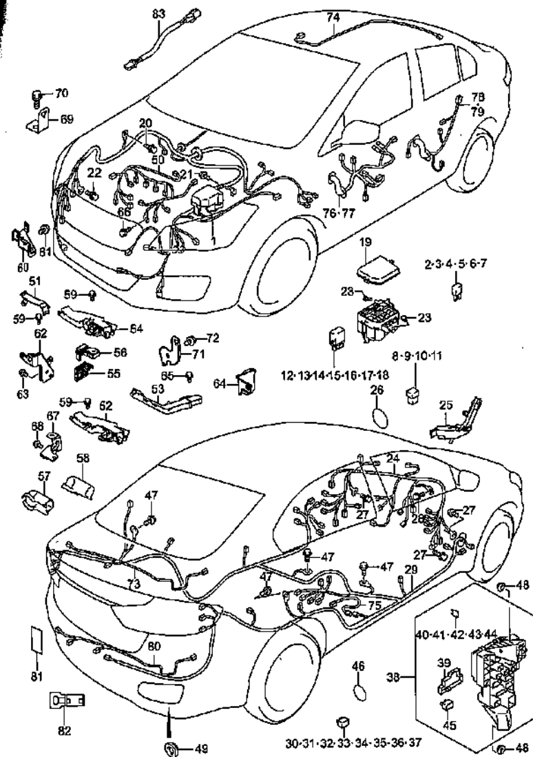
WIRING HARNESS (2)
