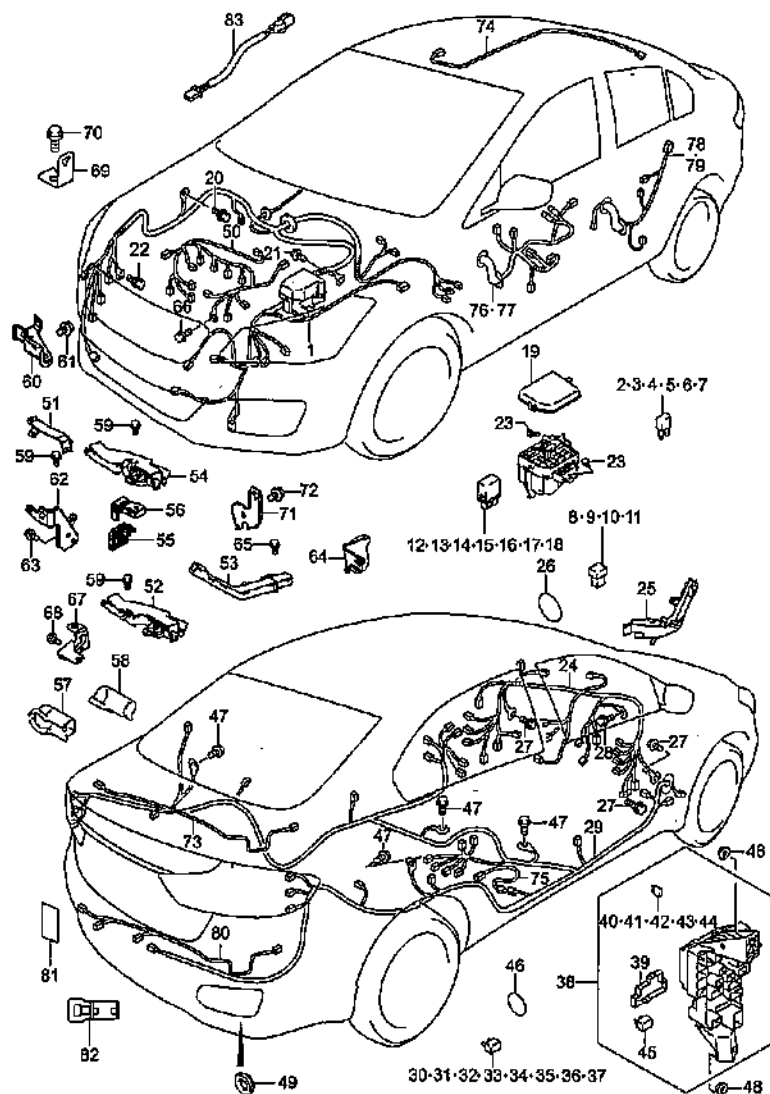
WIRING HARNESS (2)
