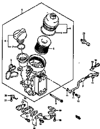
OIL FILTER
