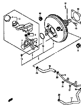
BRAKE MASTER CYLINDER (2)
