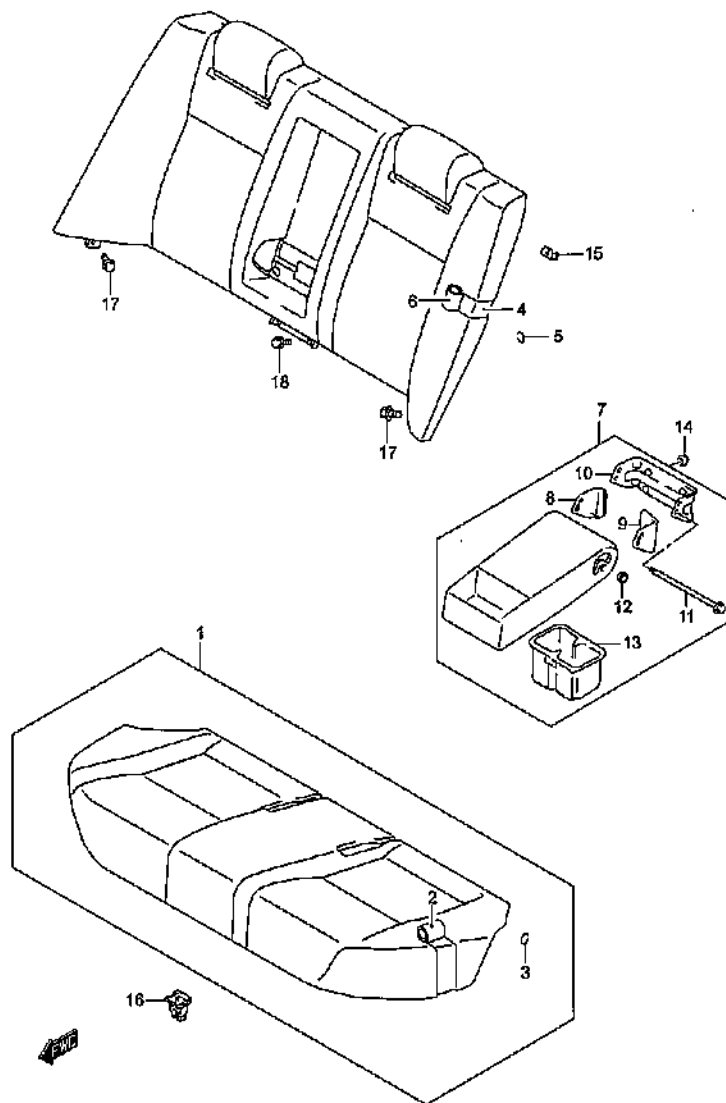
REAR SEAT
