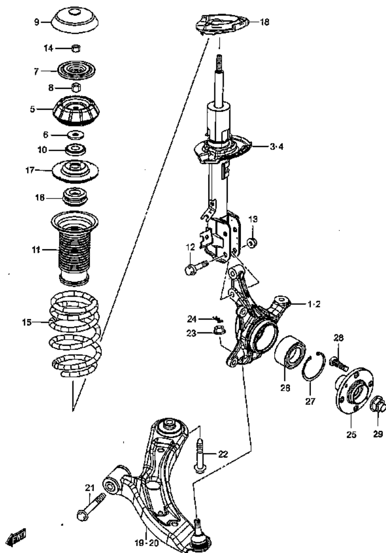
FRONT SUSPENSION
