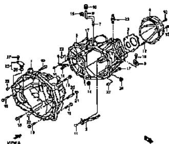
MT TRANSMISSION GEAR (3)
