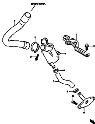
OIL SEPARATION
