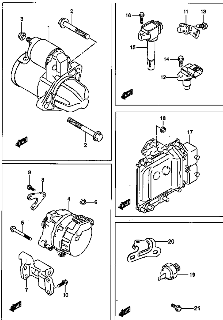
ENGINE ELECTRICAL (2)
