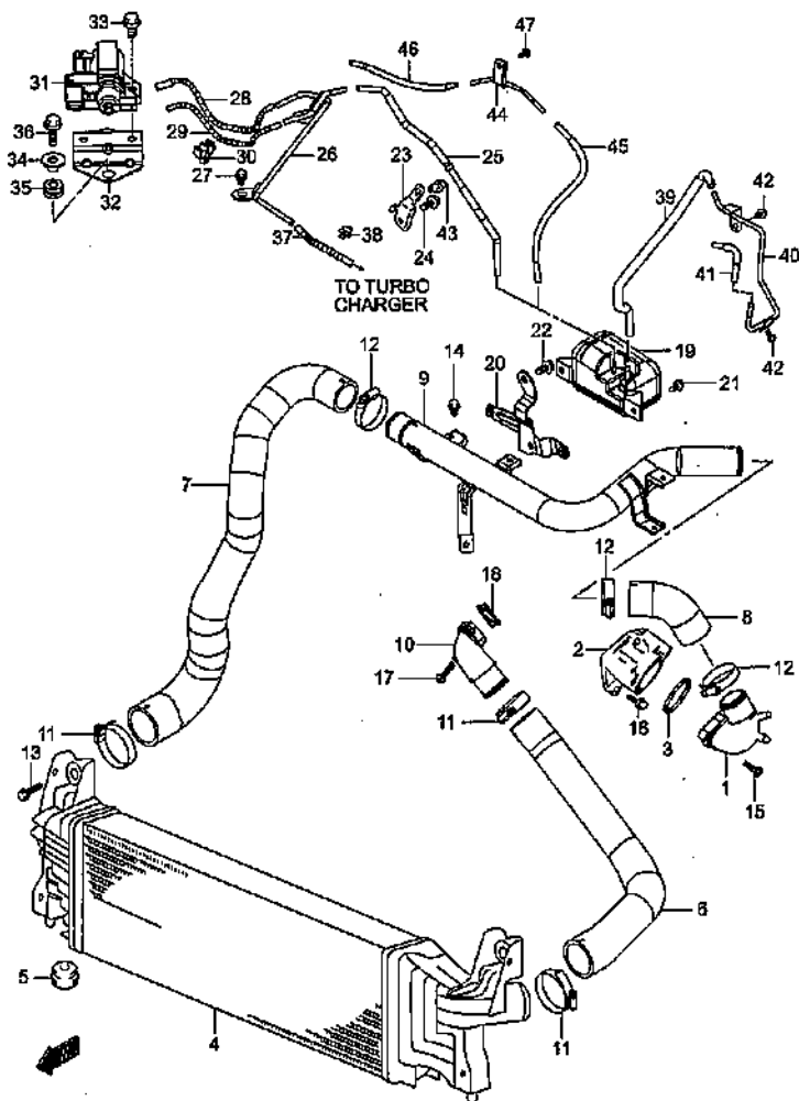
INTER COOLER
