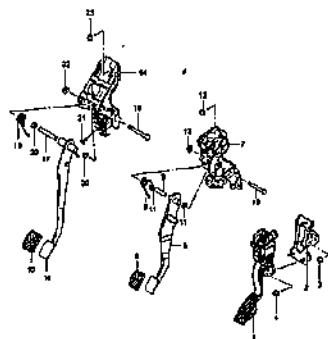
PEDAL/PEDAL BRACKET (MT)
