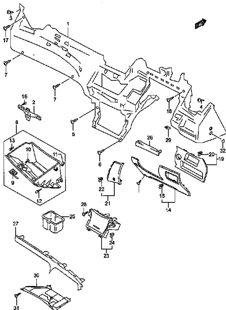
INSTRUMENT PANELL LOWER
