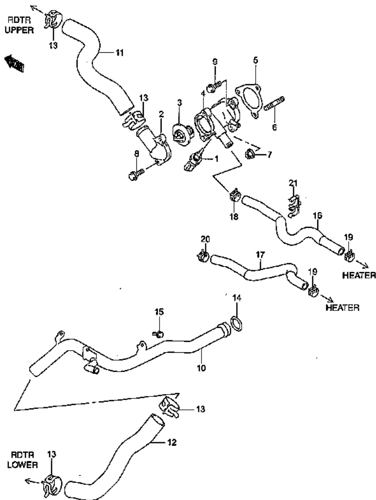
WATER HOSE (2)
