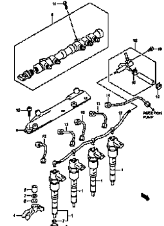
FUEL INJECTOR
