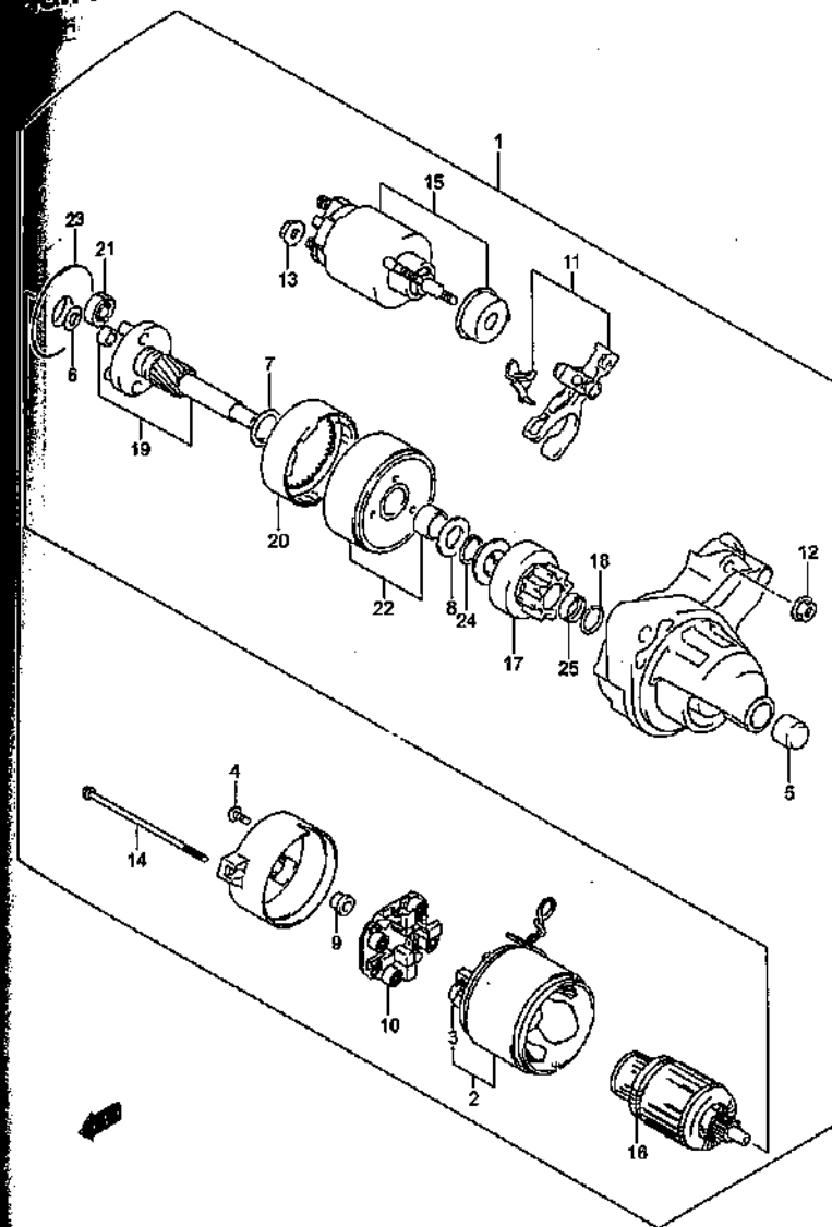
STARTING MOTOR (1)
