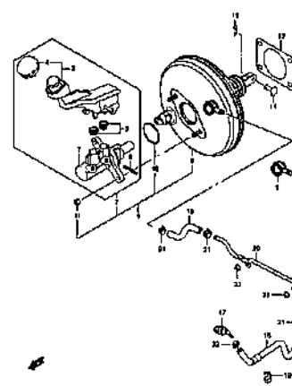
BRAKE MASTER CYLINDER (6)
