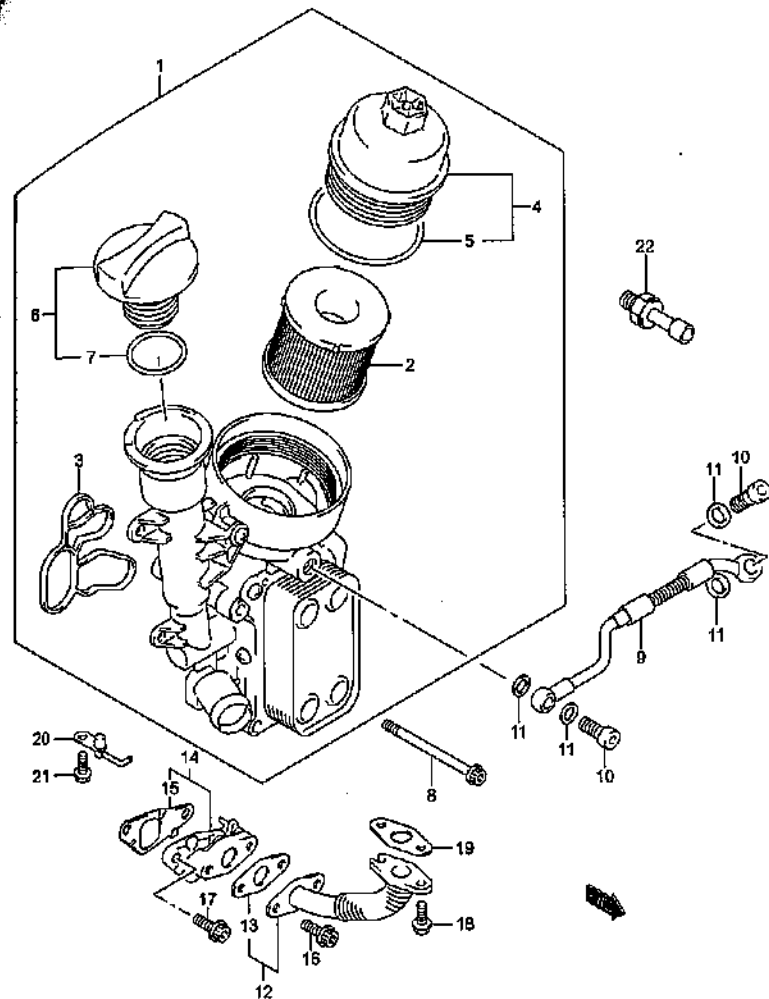
OIL FILTER
