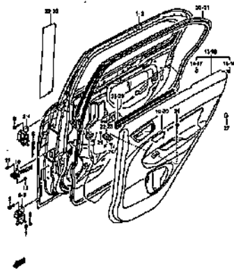
REAR DOOR PANEL
