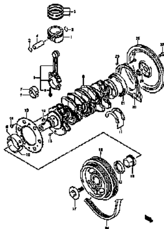
CRANKSHAFT (1)
