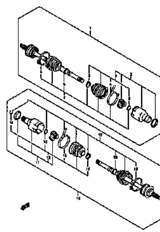
FRONT DRIVE SHAFT (3)
