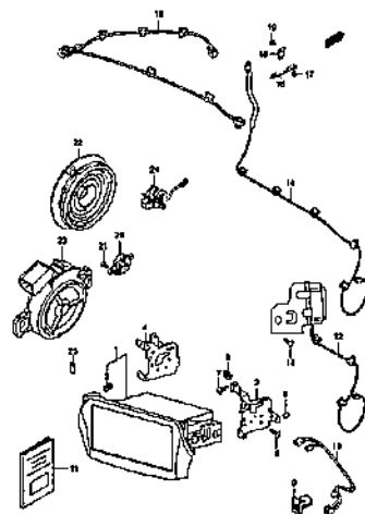
RADIO (3)
