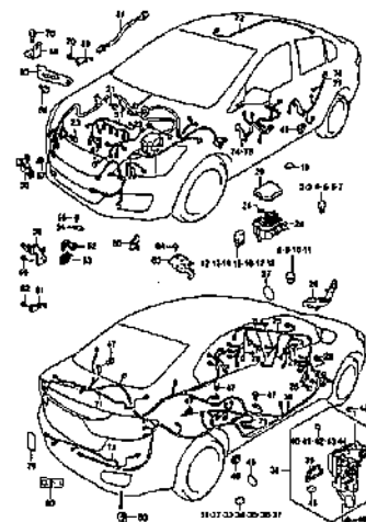
WIRING HARNESS (1)
