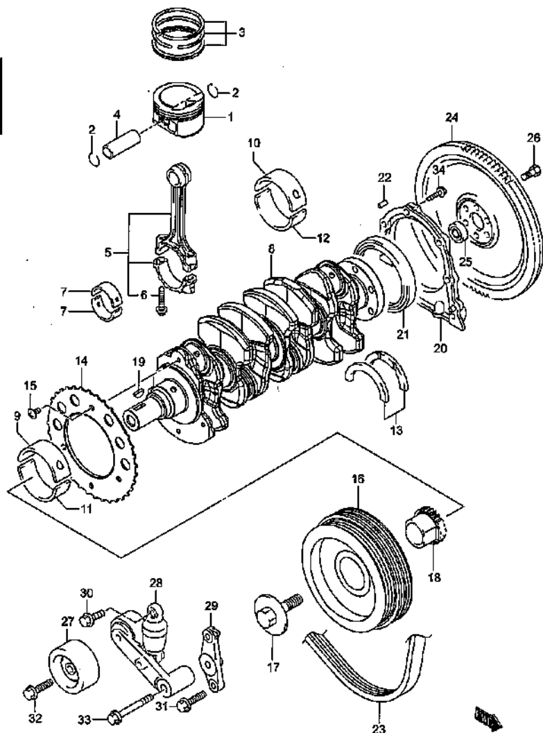
CRANKSHAFT (2)
