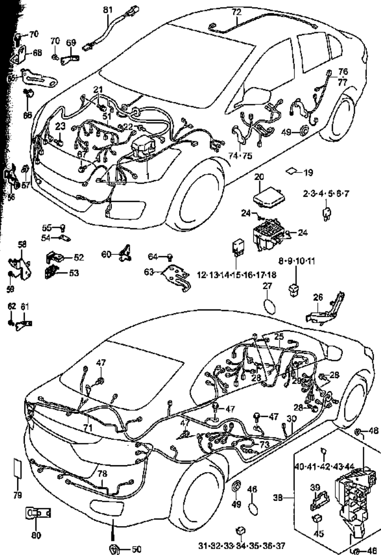
WIRING HARNESS (1)
