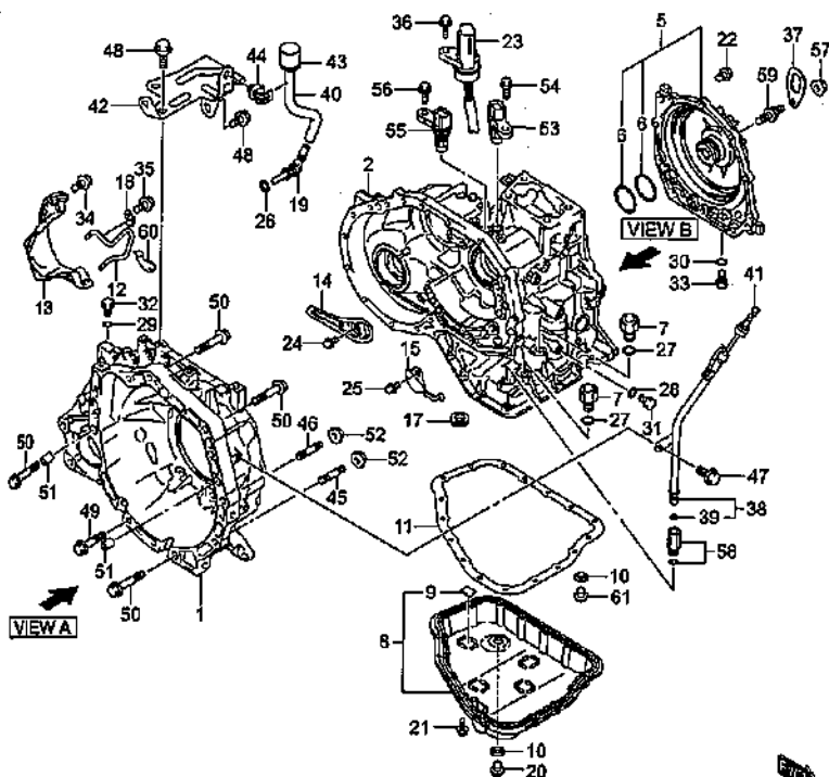
AT TRANSMISSION CASE
