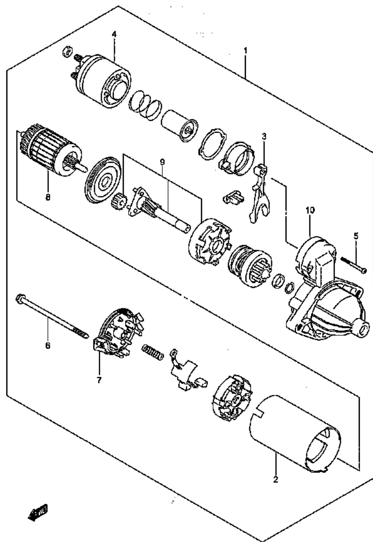
STARTING MOTOR (4)
