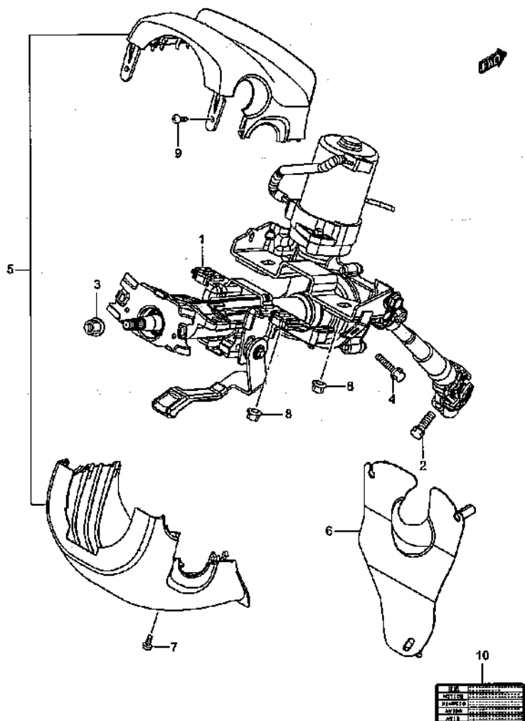
STEERING COLUMN (1)
