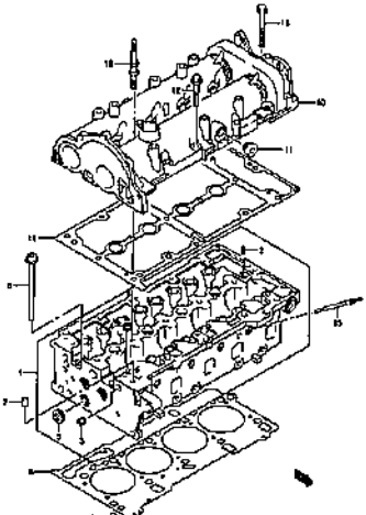
CYLINDER HEAD
