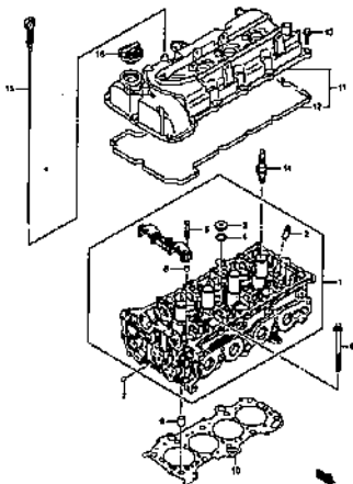
CYLINDER HEAD (2)
