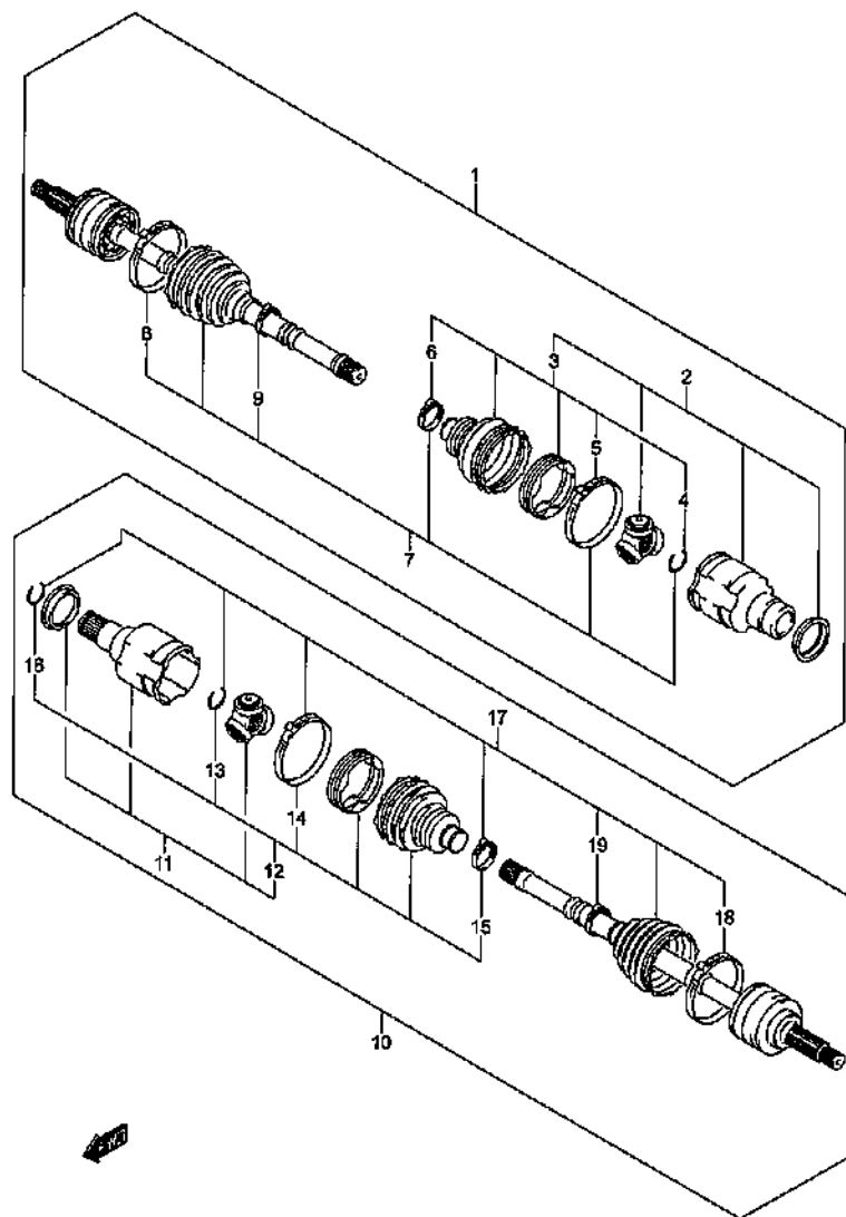
FRONT DRIVE SHAFT (2)
