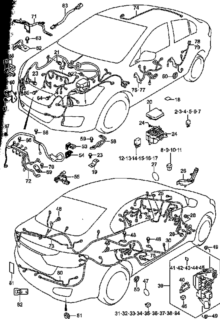
WIRING HARNESS (3)
