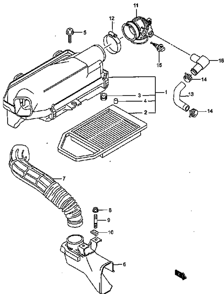
AIR CLEANER (2)
