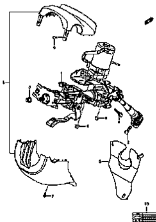
STEERING COLUMN (2)
