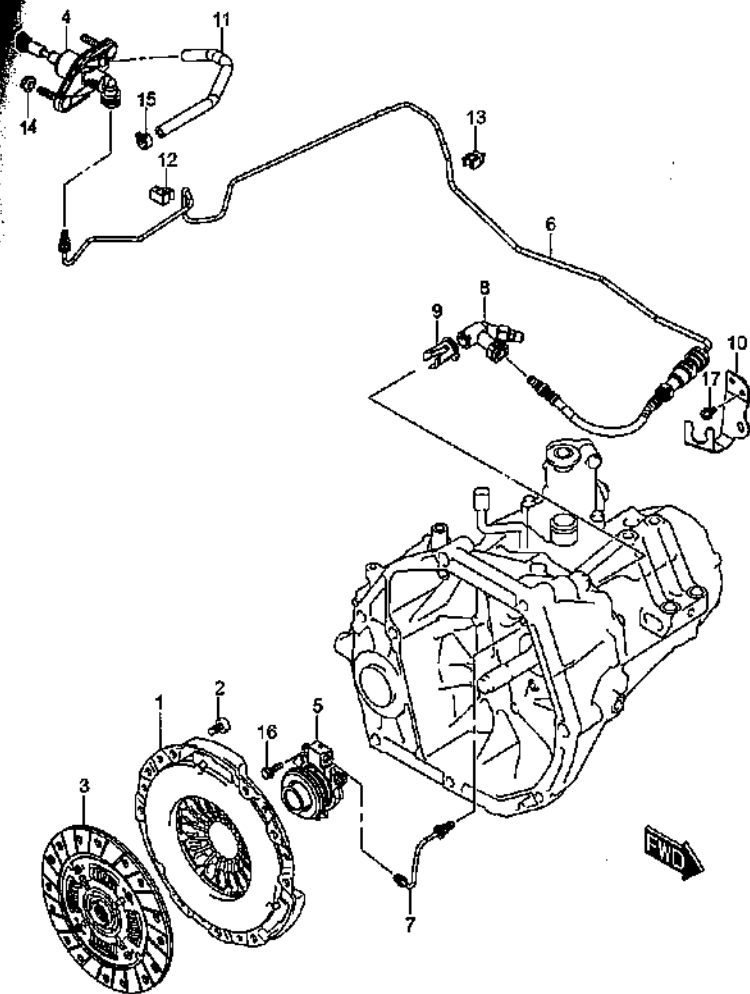
MT CLUTCH (4)
