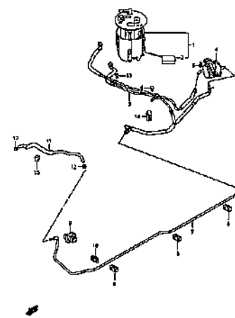
FUEL PUMP (2)
