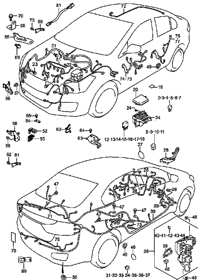
WIRING HARNESS (1)
