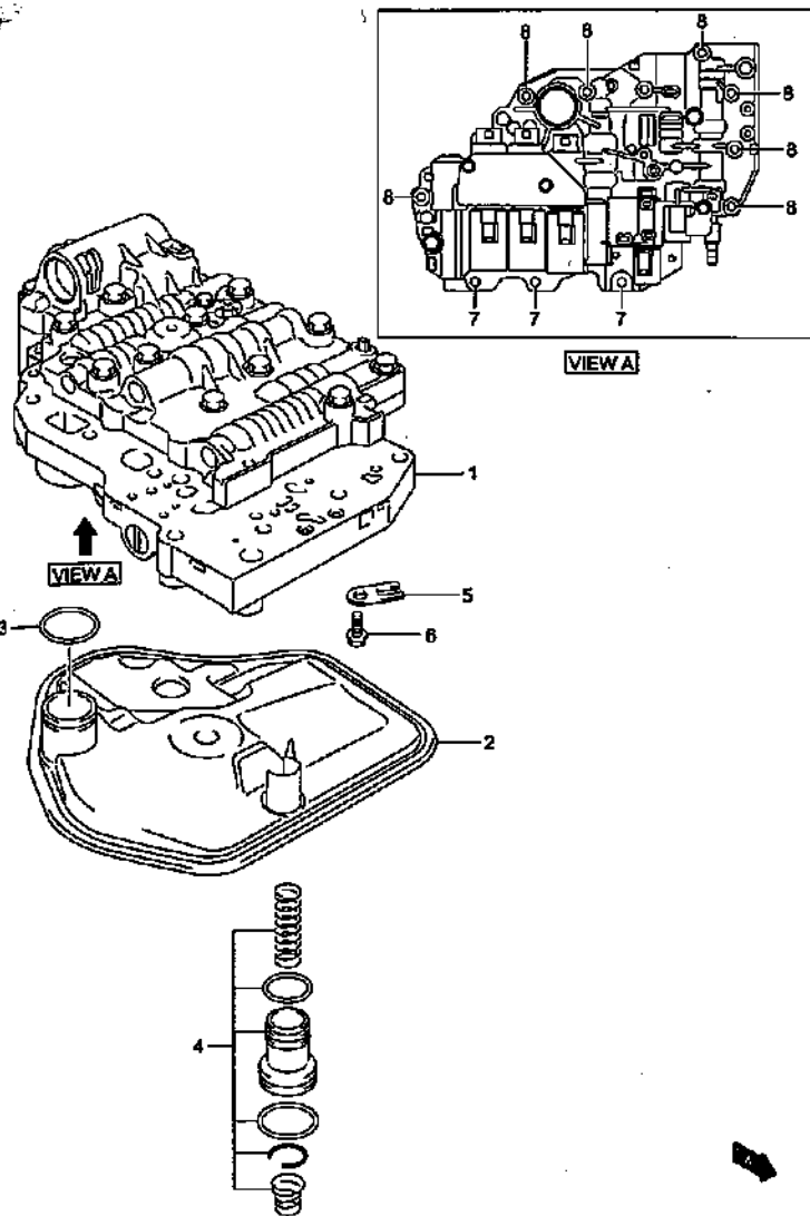
AT VALVE
