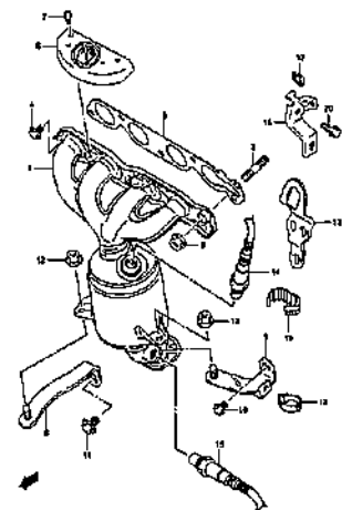
EXHAUST MANIFOLD (1)
