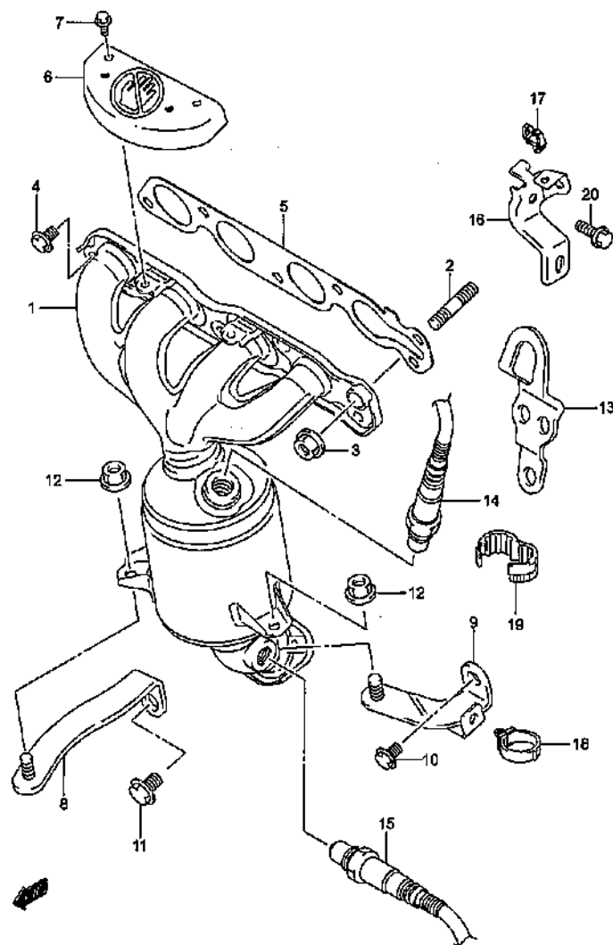
EXHAUST MANIFOLD (1)
