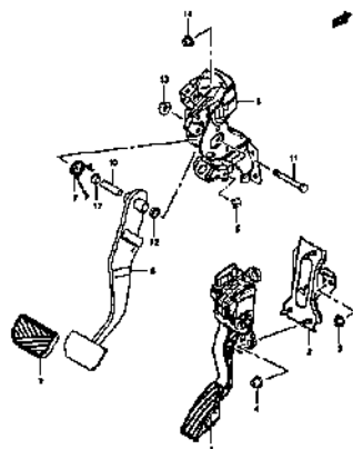
PEDAL/PEDAL BRACKET (AT)
