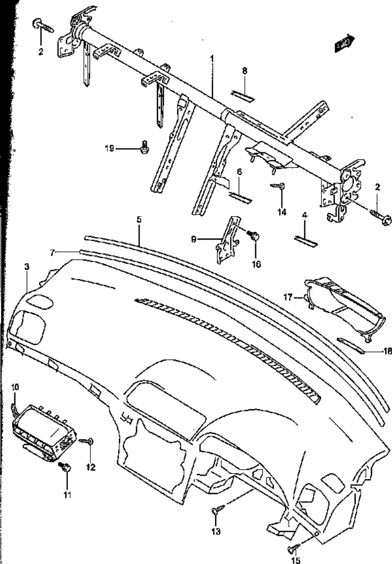
INSTRUMENT PANEL UPPER
