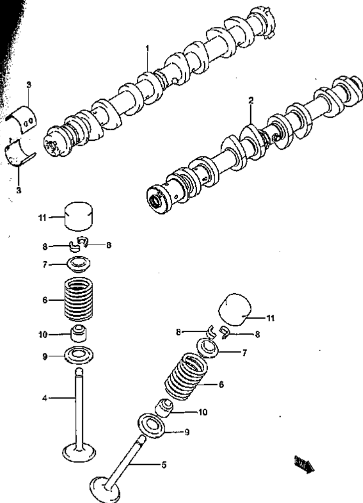
CAM SHAFT/VALVE (2)
