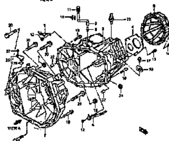
MT TRANSMISSION CASE (2)
