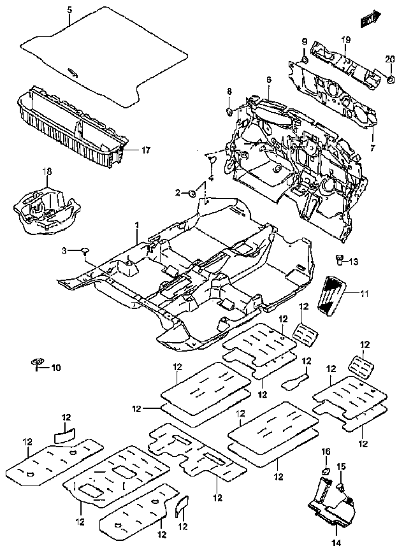
FLOOR CARPET
