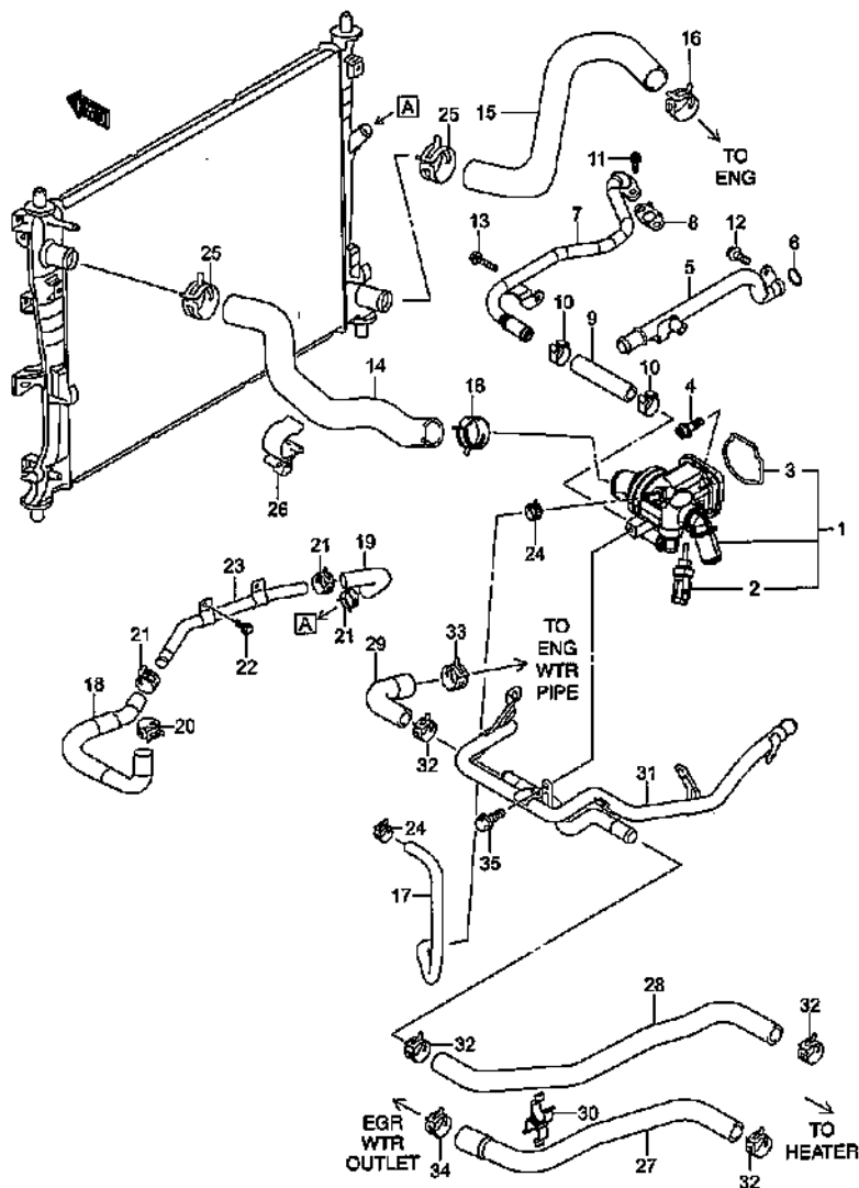
WATER HOSE (2)
