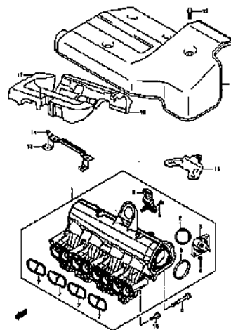
INTAKE MANIFOLD (3)
