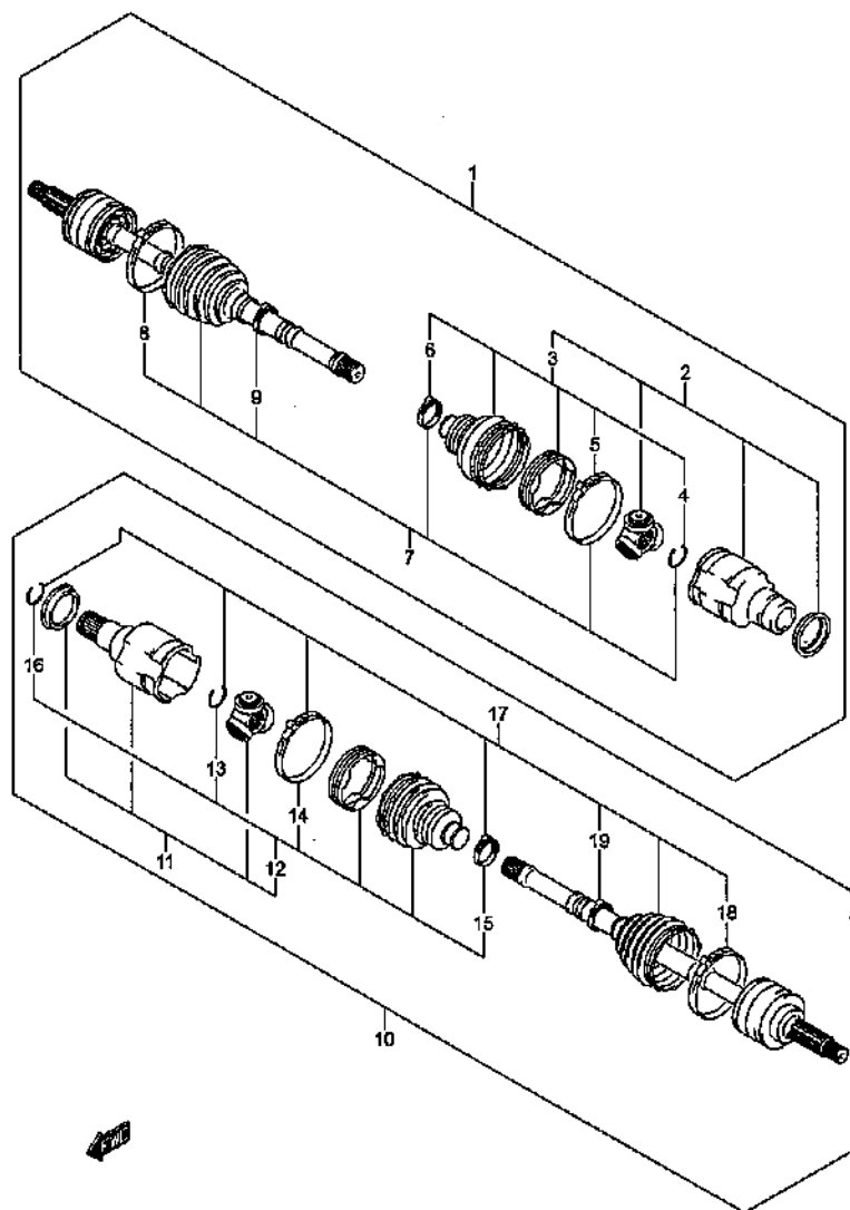
FRONT DRIVE SHAFT (5)
