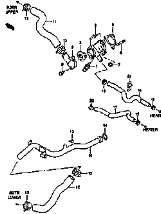
WATER HOSE (2)
