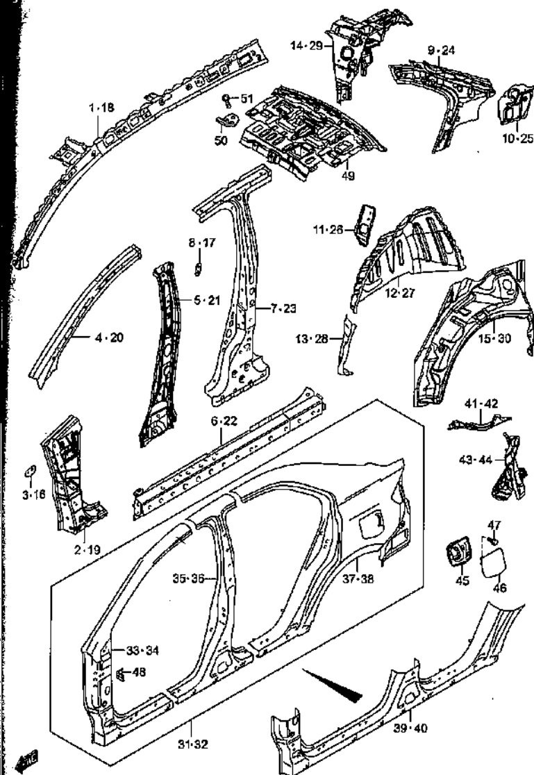
SIDE BODY PANEL
