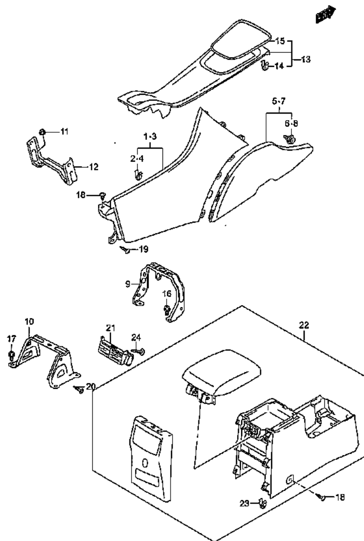
CONSOLE BOX
