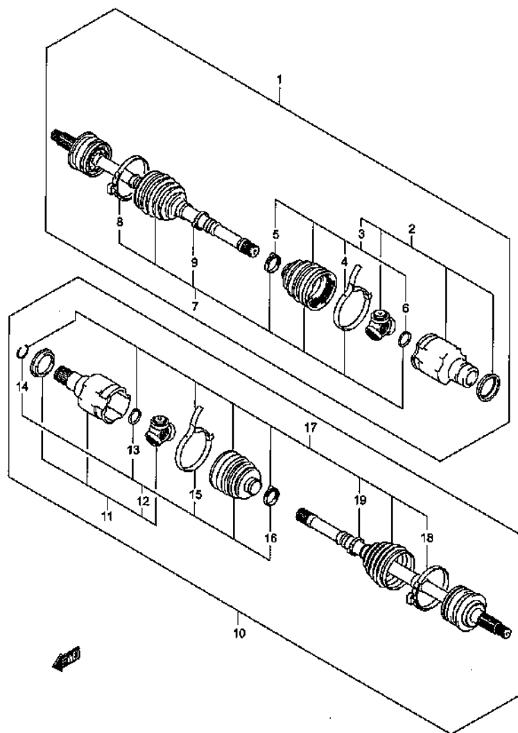
FRONT DRIVE SHAFT (3)
