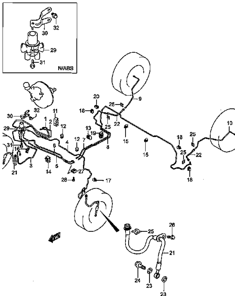
BRAKE PIPING (N/ABS)
