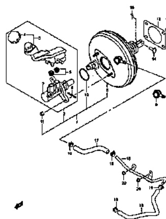
BRAKE MASTER CYLINDER (4)
