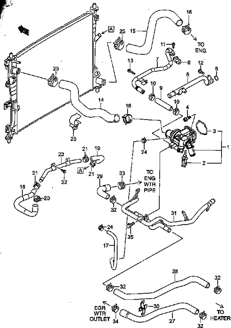
WATER HOSE (2)
