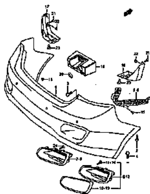
REAR BUMPER (2)
