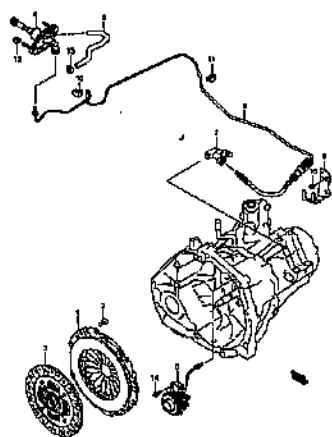
MT CLUTCH (3)
