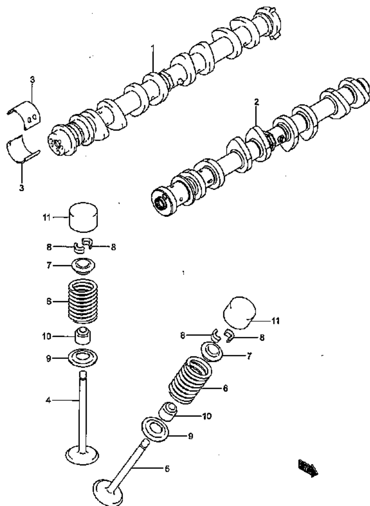
CAM SHAFT/VALVE (2)
