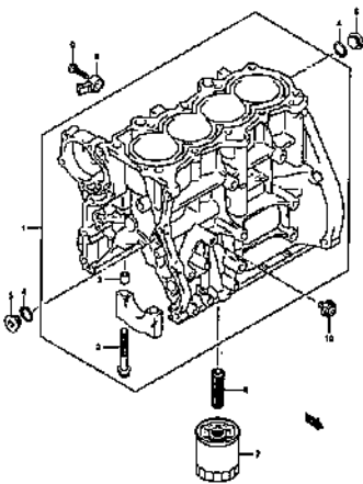
CYLINDER
