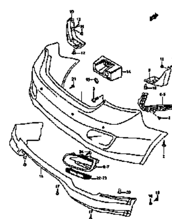
REAR BUMPER
