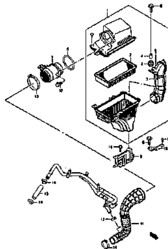
AIR CLEANER (3)
