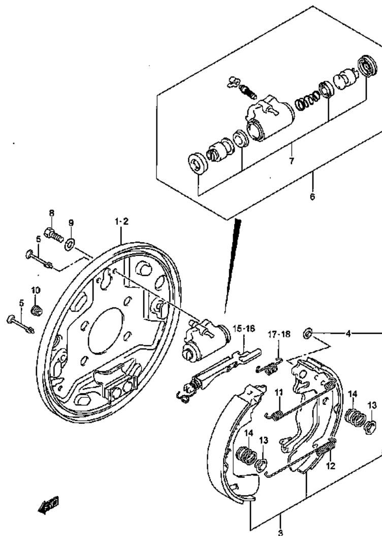
REAR WHEEL BRAKE
