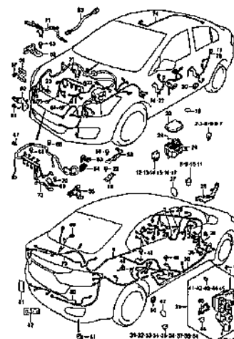
WIRING HARNESS (3)
