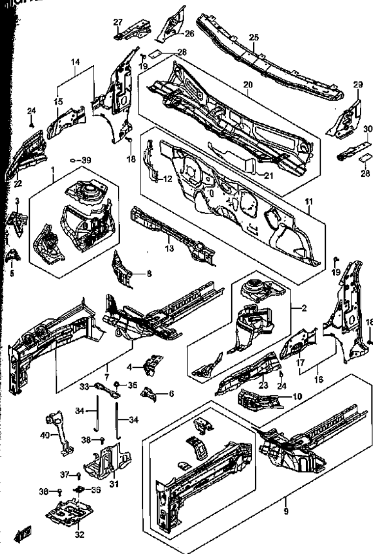
FRONT BODY PANEL
