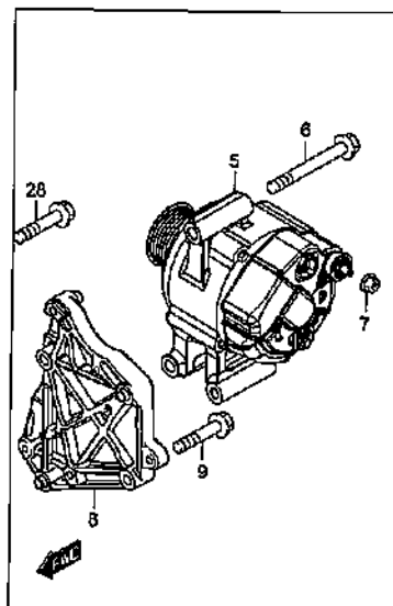
ENGINE ELECTRICAL (3)
