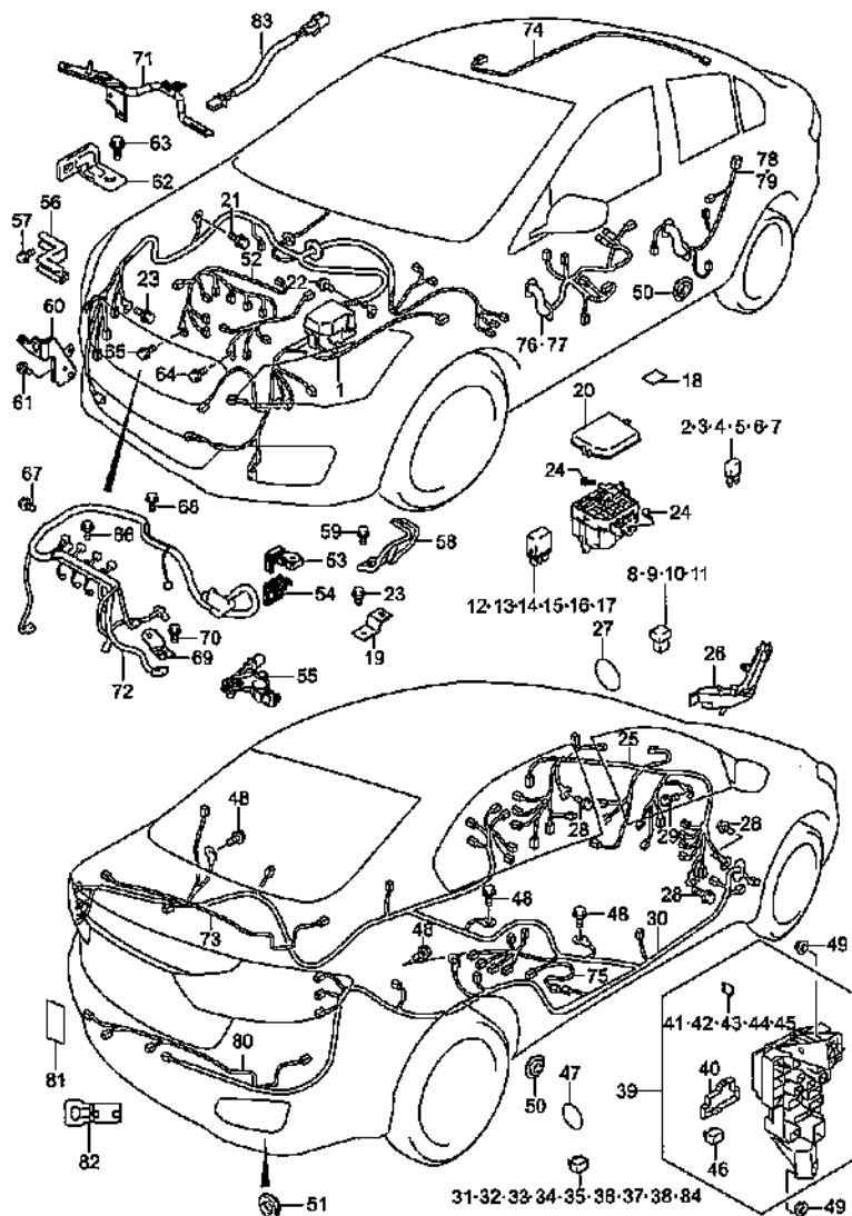
WIRING HARNESS (3)
