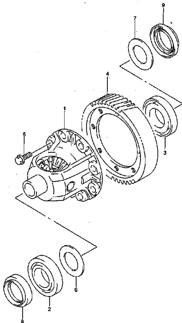
FRONT DIFFERENTIAL GEAR (2)
