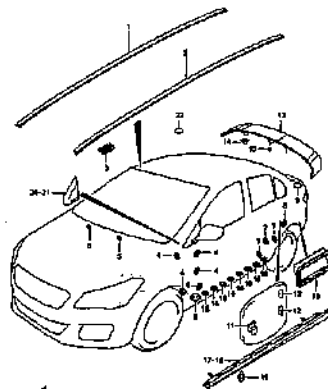
ROOF MOLDING
