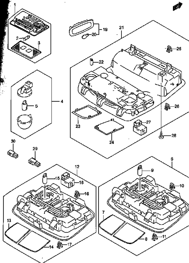
ROOM LAMP
