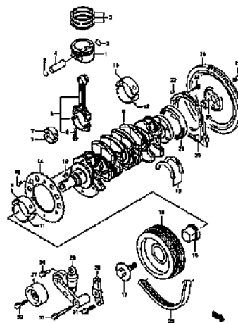
CRANKSHAFT (2)
