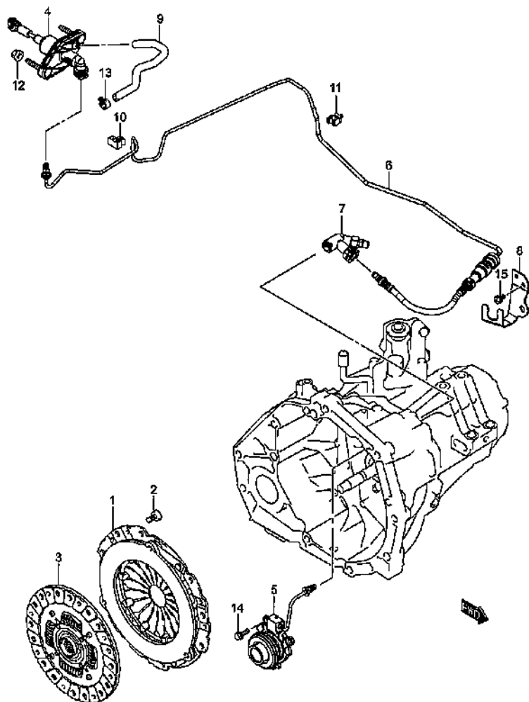
MT CLUTCH (1)
