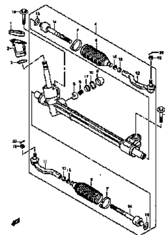
STEERING UNIT
