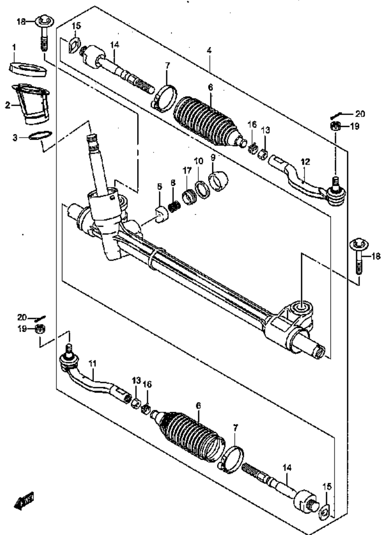
STEERING UNIT
