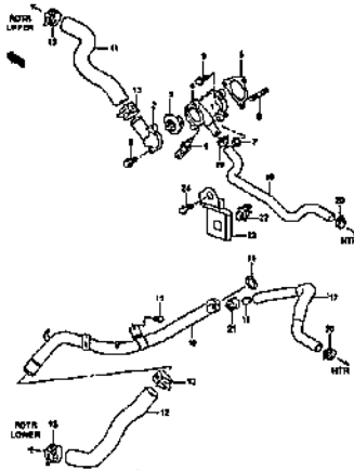
WATER HOSE (1)
