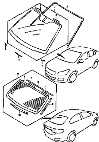
FRONT/BACK GLASS
