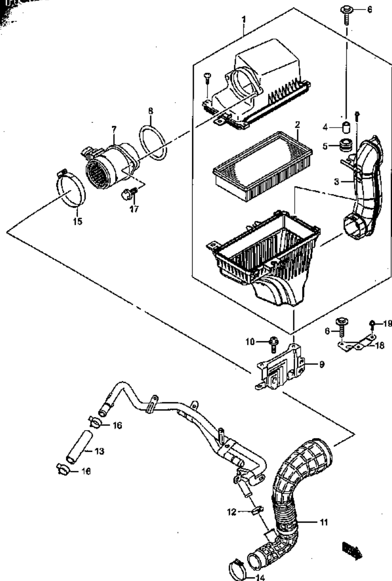
AIR CLEANER (2)
